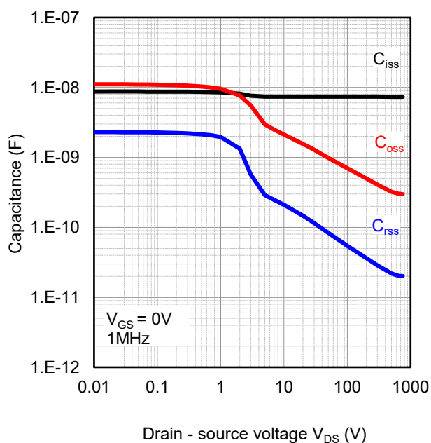
Figure 23. Capacitance vs. Drain - source voltage at 25°C (Typ.)
