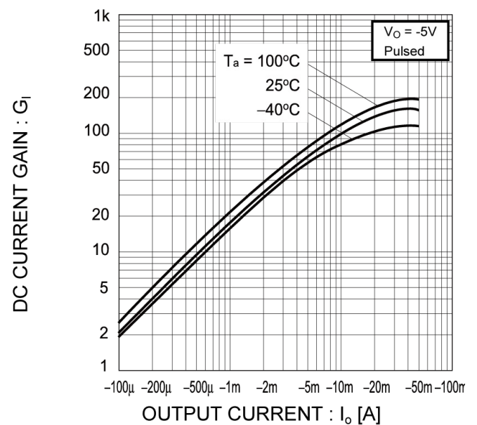
Fig.4 DC current gain vs. output current
