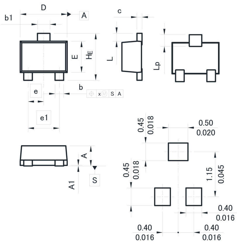
Soldering footprint
