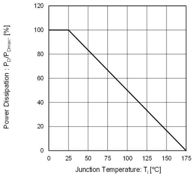
Fig.1 Power Dissipation Derating Curve
