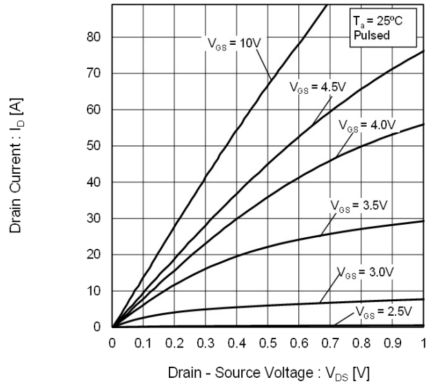
Fig.5 Typical Output Characteristics(I)
