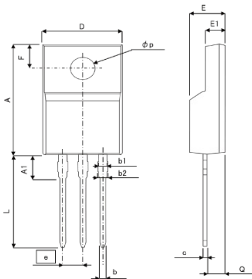
TO-220FM
