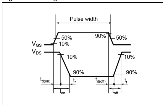
Fig.1-2 Switching Waveforms
