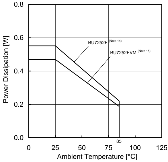
(e) BU7252xxx
