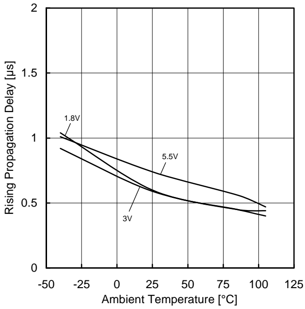
Figure 21. Rising Propagation Delay vs Ambient Temperature ( C_L=15\text{pF} , 100mV Overdrive)
