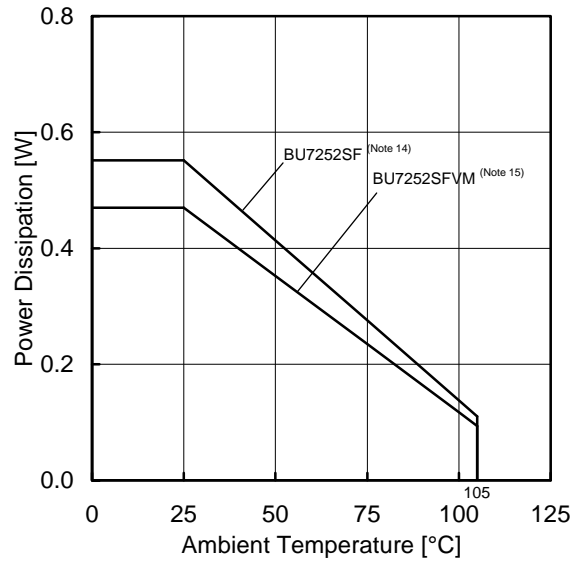
(f) BU7252Sxxx
