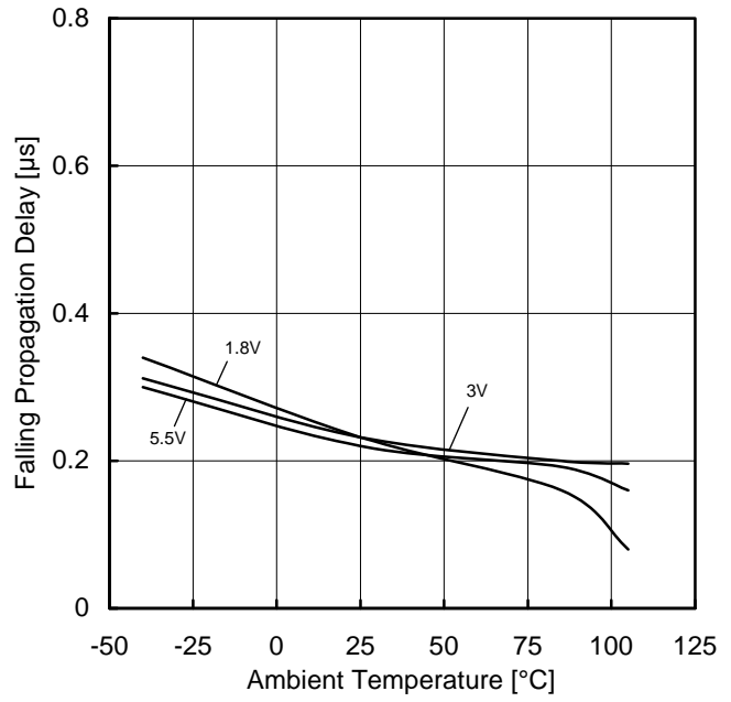
Figure 44. Falling Propagation Delay vs Ambient Temperature ( C_L=15\text{pF} , 100mV Overdrive)
