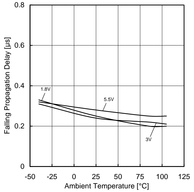
Figure 22. Falling Propagation Delay vs Ambient Temperature ( C_L=15\text{pF} , 100mV Overdrive)
