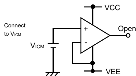
Figure 20. Example of application unused circuit processing
