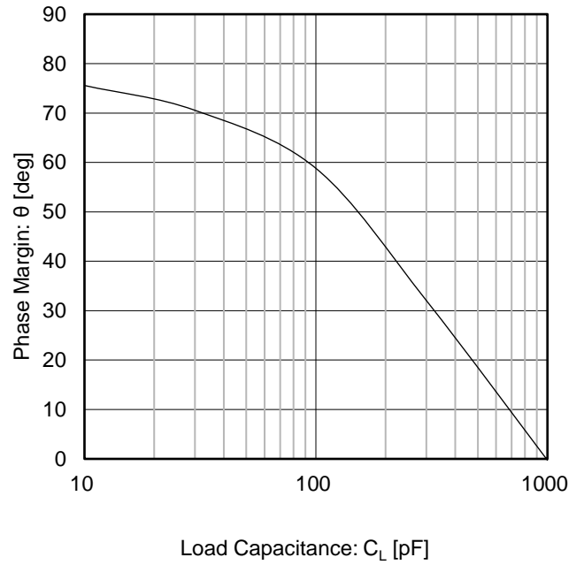
Figure 30. Phase Margin vs Load Capacitance ( V_S = 5\text{ V} , R_F = 10\text{ k}\Omega , G = 40\text{ dB} )
