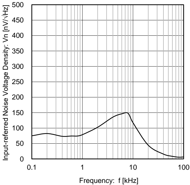
Figure 23. Input-referred Noise Voltage Density vs Frequency ( V_s = 2.7\text{ V} )
