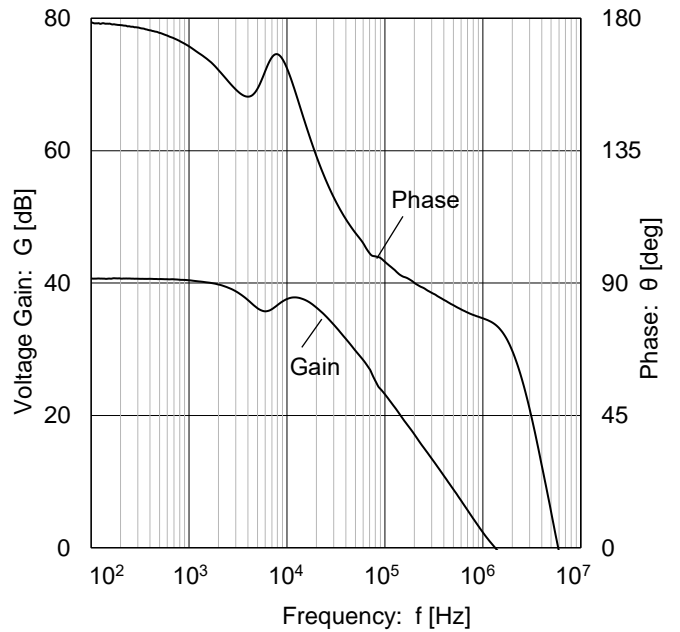
Figure 32. Voltage Gain, Phase vs Frequency ( V_S = 5\text{ V} )
