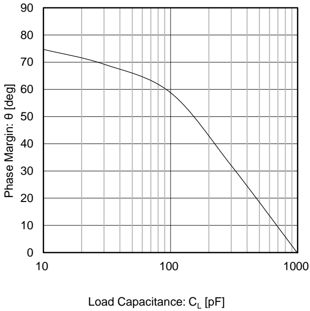
Figure 29. Phase Margin vs Load Capacitance ( V_S = 2.7\text{ V} , R_F = 10\text{ k}\Omega , G = 40\text{ dB} )
