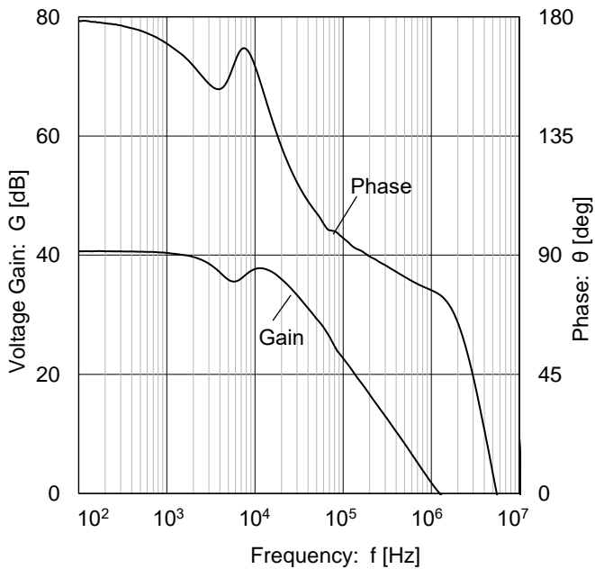
Figure 31. Voltage Gain, Phase vs Frequency ( V_S = 2.7\text{ V} )
