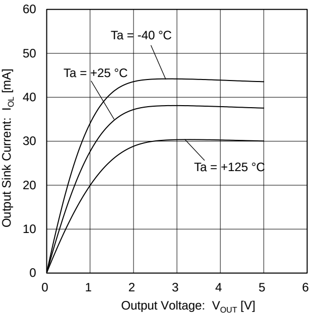
Figure 10. Output Sink Current vs Output Voltage (V S = 5.0 V)
