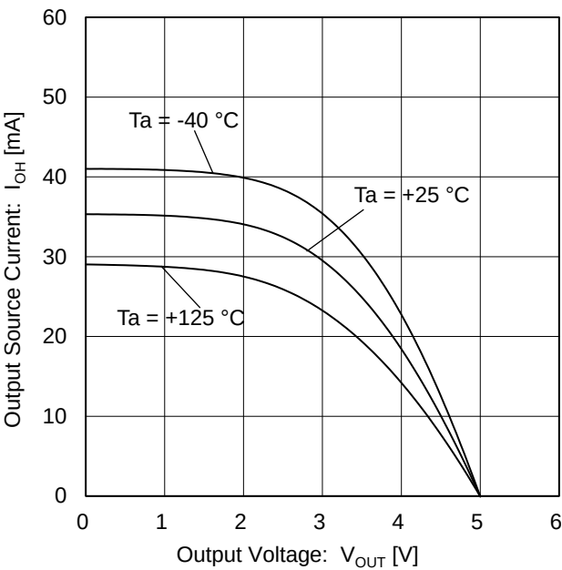
Figure 9. Output Source Current vs Output Voltage (V S = 5.0 V)
