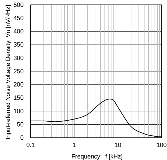
Figure 23. Input-referred Noise Voltage Density vs Frequency (V S = 5.0 V)
