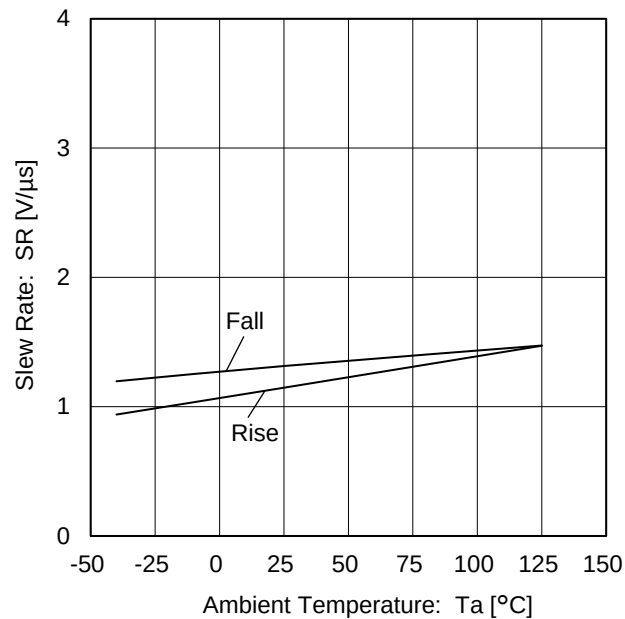
Figure 22. Slew Rate vs Ambient Temperature (V S = 5.0 V)
