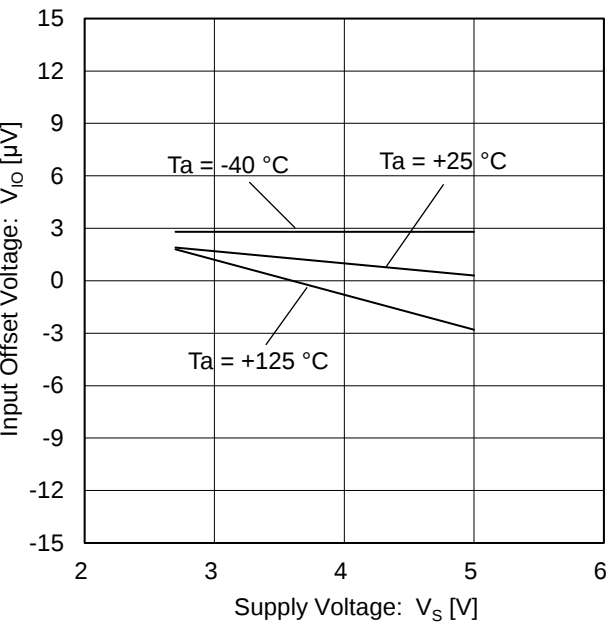
Figure 11. Input Offset Voltage vs Supply Voltage (V ICM = 0 V)
