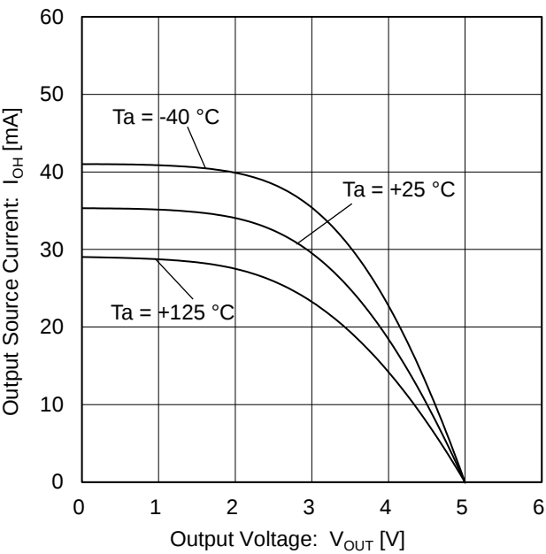
Figure 9. Output Source Current vs Output Voltage (V S = 5 V)
