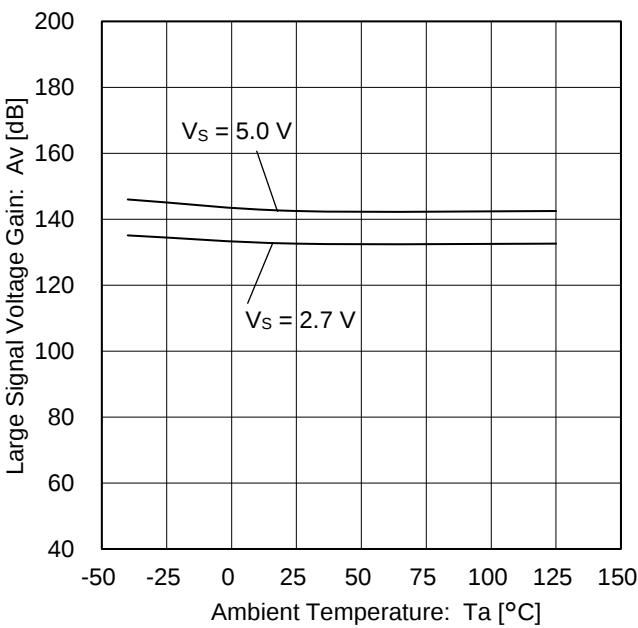
Figure 18. Large Signal Voltage Gain vs Ambient Temperature
