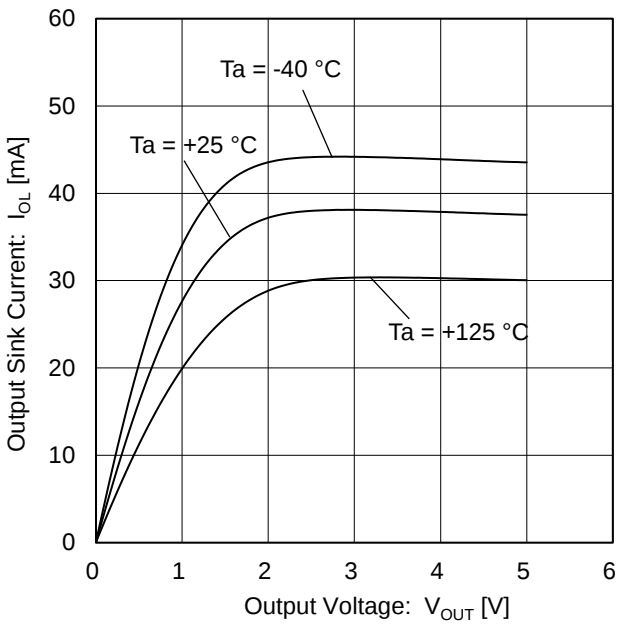
Figure 10. Output Sink Current vs Output Voltage (V S = 5 V)
