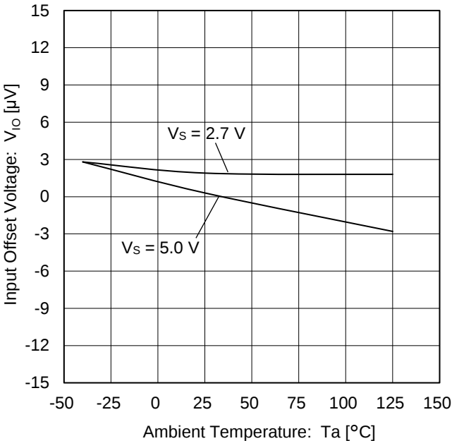
Figure 12. Input Offset Voltage vs Ambient Temperature (V ICM = 0 V)
