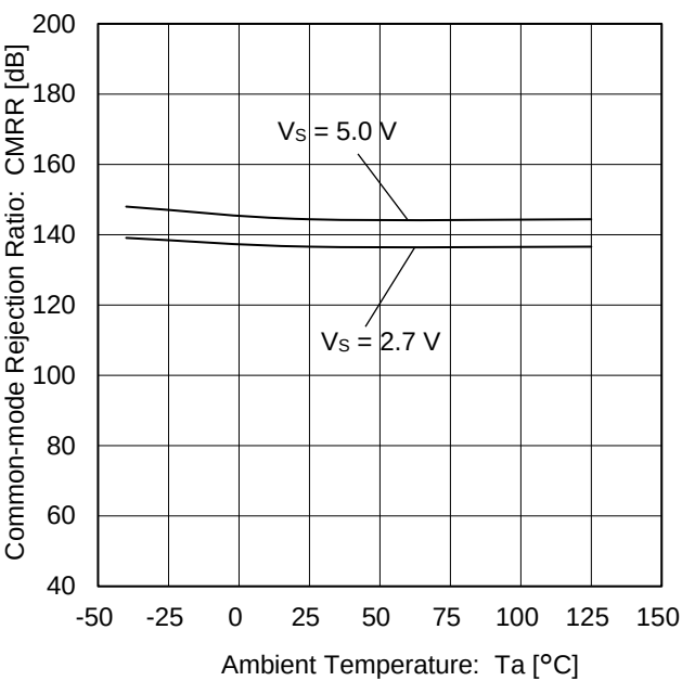
Figure 18. Common-mode Rejection Ratio vs Ambient Temperature
