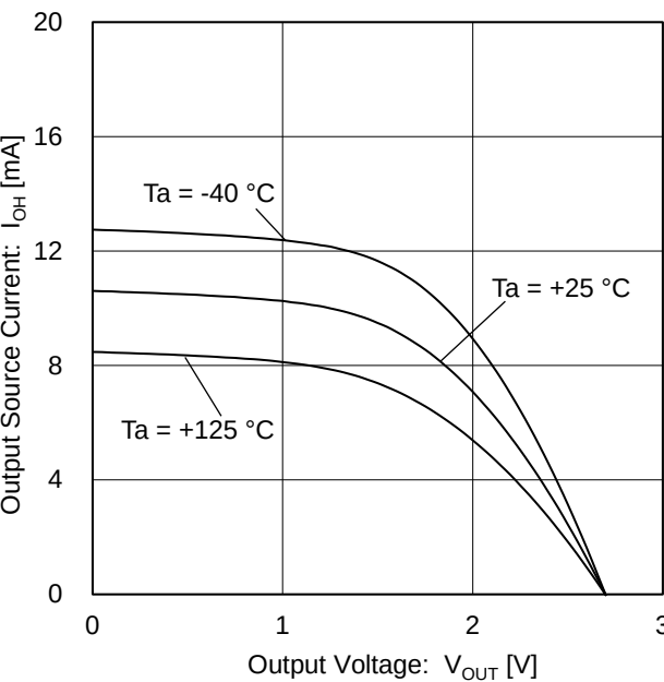
Figure 7. Output Source Current vs Output Voltage ( V_S = 2.7\text{ V} )
