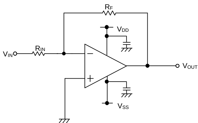
Figure 25. Inverting Amplifier Circuit
