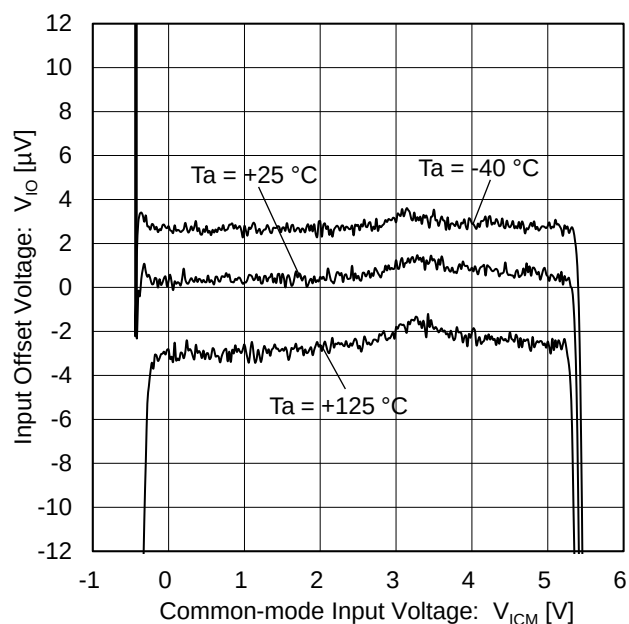
Figure 14. Input Offset Voltage vs Common-mode Input Voltage ( V_S = 5.0\text{ V} )
