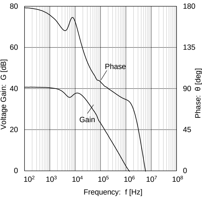
Figure 20. Voltage Gain, Phase vs Frequency ( V_S = 5.0\text{ V} )
