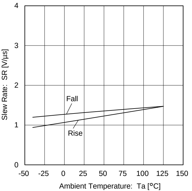
Figure 22. Slew Rate vs Ambient Temperature ( V_S = 5.0\text{ V} )
