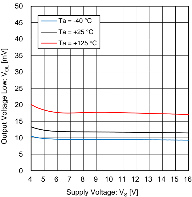
Figure 5. Output Voltage Low vs Supply Voltage (I L = 1 mA)
