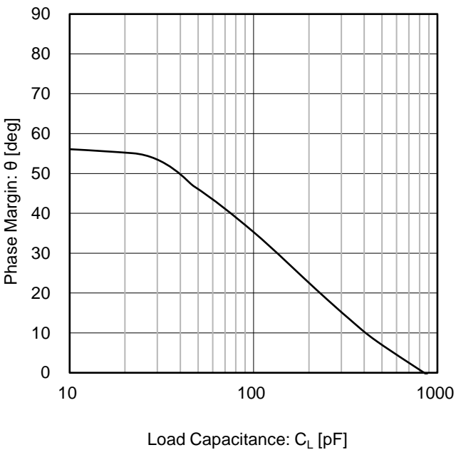
Figure 26. Phase Margin vs Load Capacitance (V S = 10 V, R F = 10 kΩ, G = 40 dB)
