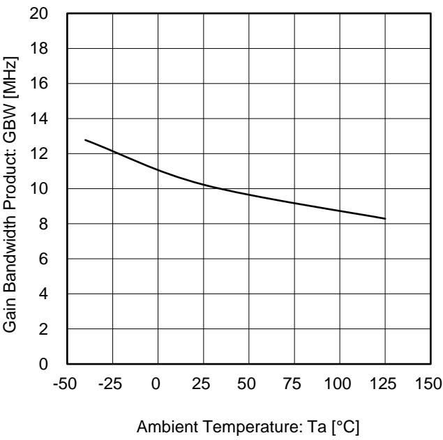
Figure 25. Gain Bandwidth Product: vs Ambient Temperature (V S = 10 V, R F = 10 kΩ, G = 40 dB)
