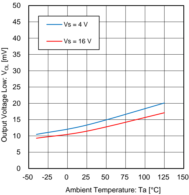
Figure 6. Output Voltage Low vs Ambient Temperature (I L = 1 mA)
