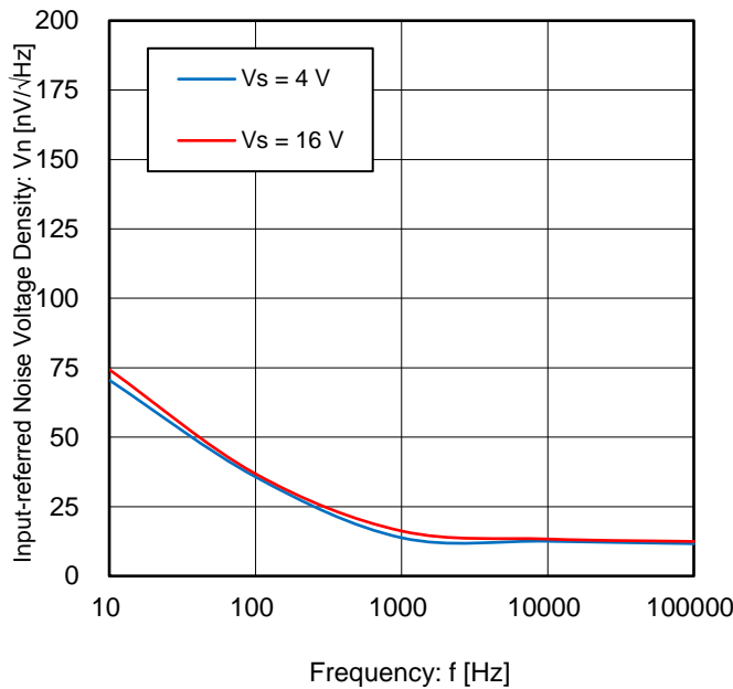
Figure 21. Input-referred Noise Voltage Density vs Frequency
