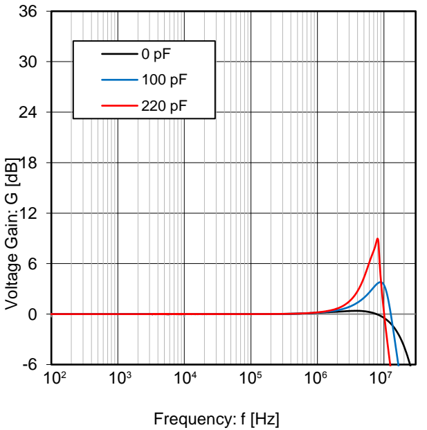
Figure 28. Voltage Gain vs Frequency (V S = 10 V, G = 0 dB, V IN = 180 mVp-p)
