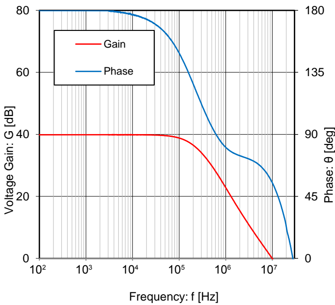
Figure 27. Voltage Gain, Phase vs Frequency (V S = 10 V, R F = 10 kΩ, G = 40 dB)
