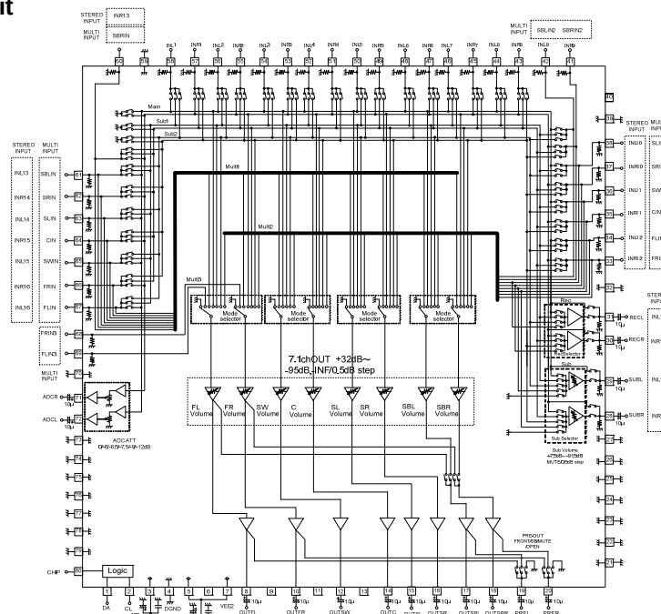
Figure 1. Application Circuit
