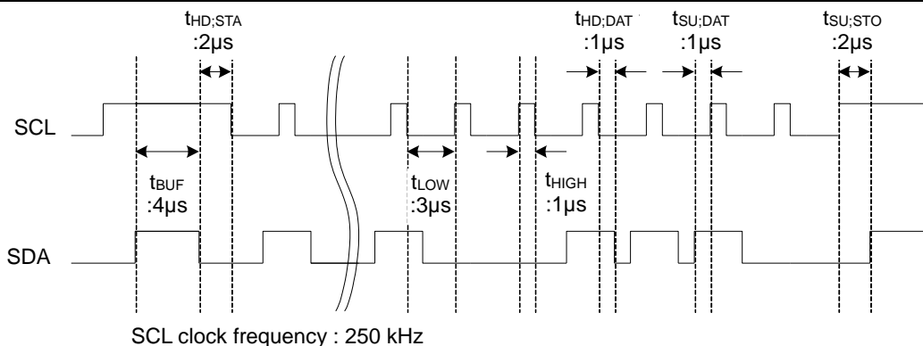
Figure 23. A Command Timing Example in the I²C Data Transmission
