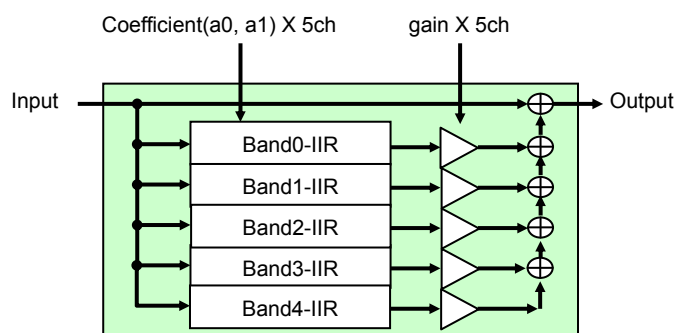
Parallel connection Figure 29
