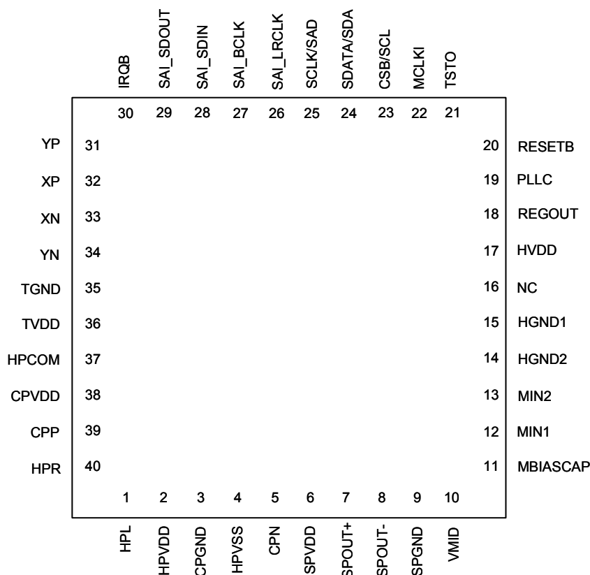
Figure 2. Pin Configuration(s)
