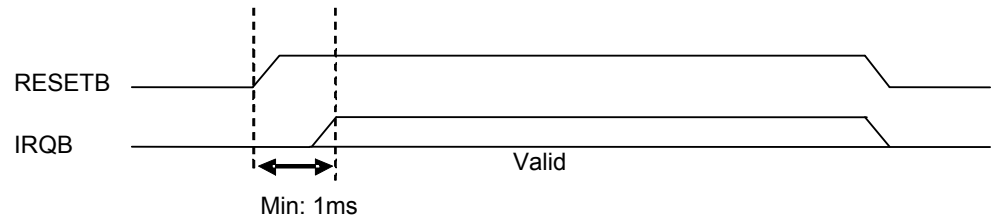
Interrupt timing Figure 40
