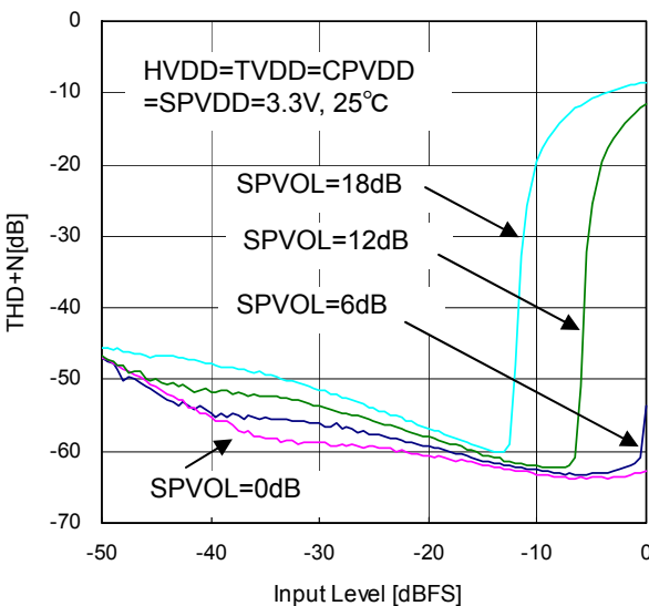
Figure 48. DAC input Level [dBFS] vs SPAMP-AB Class THD+N [dB]
