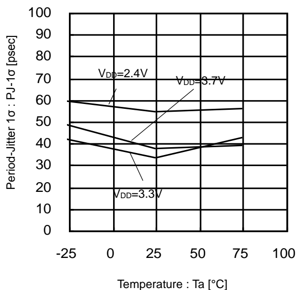
Figure 25. Period-Jitter 1 \sigma vs Temperature (36.9MHz)
