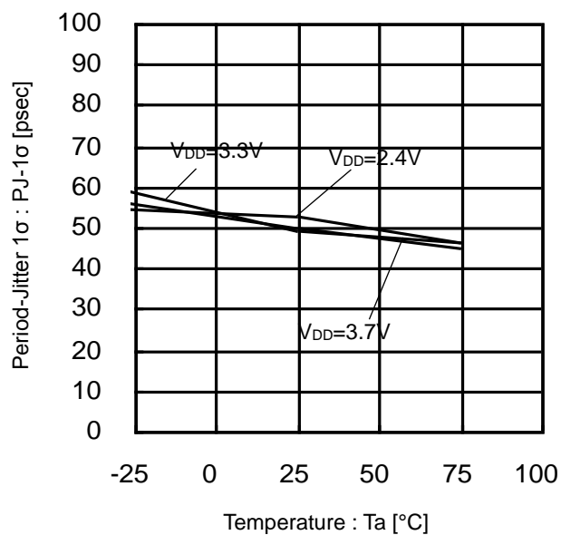
Figure 37. Period-Jitter 1 \sigma vs Temperature (27MHz)
