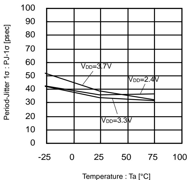
Figure 28. Period-Jitter 1 \sigma vs Temperature (22.6MHz)
