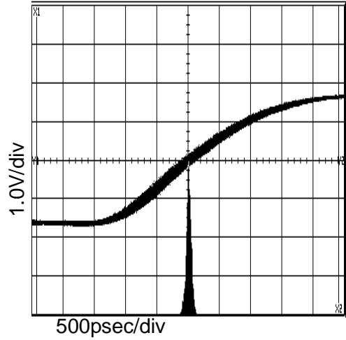
Figure 2. 54MHz Period-Jitter ( V_{DD}=3.3V , at C_L=15pF )
