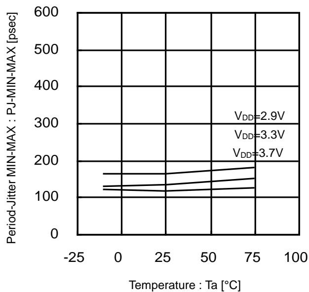
Figure 21. Period-Jitter MIN-MAX vs Temperature (30MHz)
