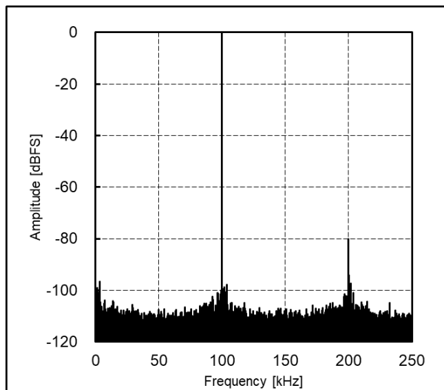
Figure 12. Amplitude vs Frequency ( V_{\text{IOVDD}} = 3\text{ V} , V_{\text{DD}} = 5\text{ V} , f_{\text{SCK}} = 10\text{ MHz} , f_s = 500\text{ kSPS} )
