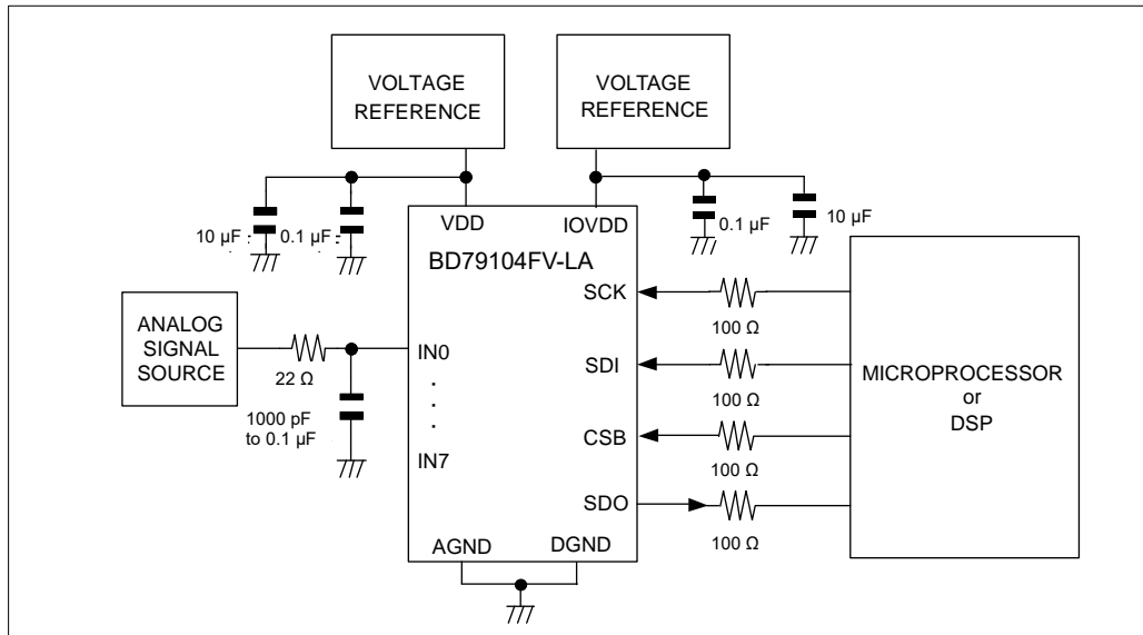
Figure 19. Application Circuit
