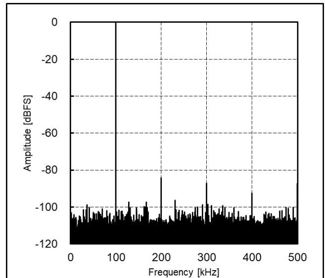
Figure 13. Amplitude vs Frequency ( V_{\text{IOVDD}} = 3\text{ V} , V_{\text{DD}} = 5\text{ V} , f_{\text{SCK}} = 20\text{ MHz} , f_s = 1\text{ MSPS} )
