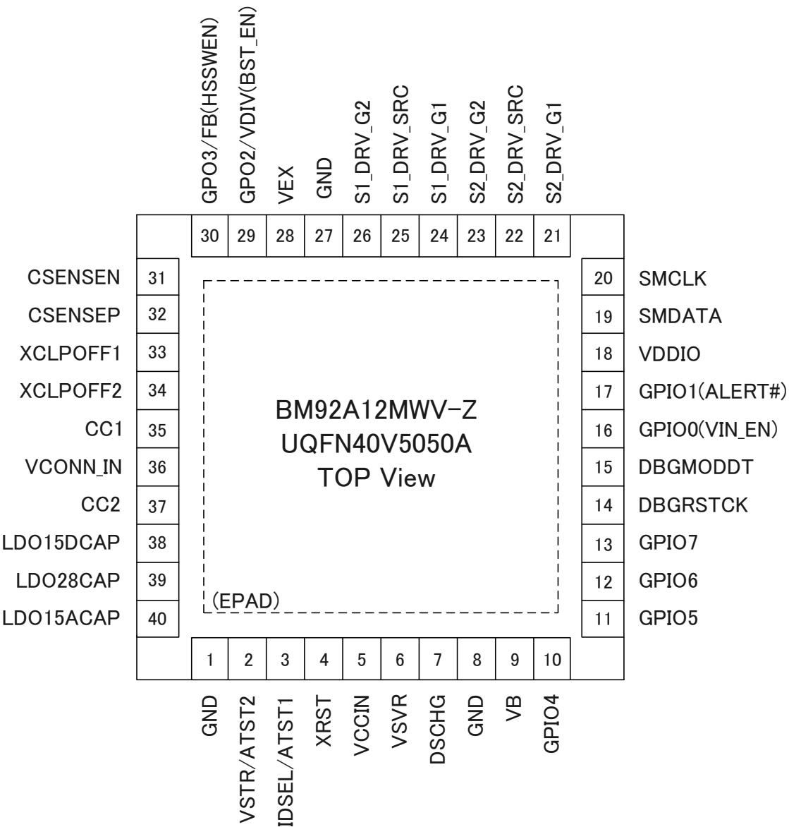
Figure 1-1 Pin configuration
