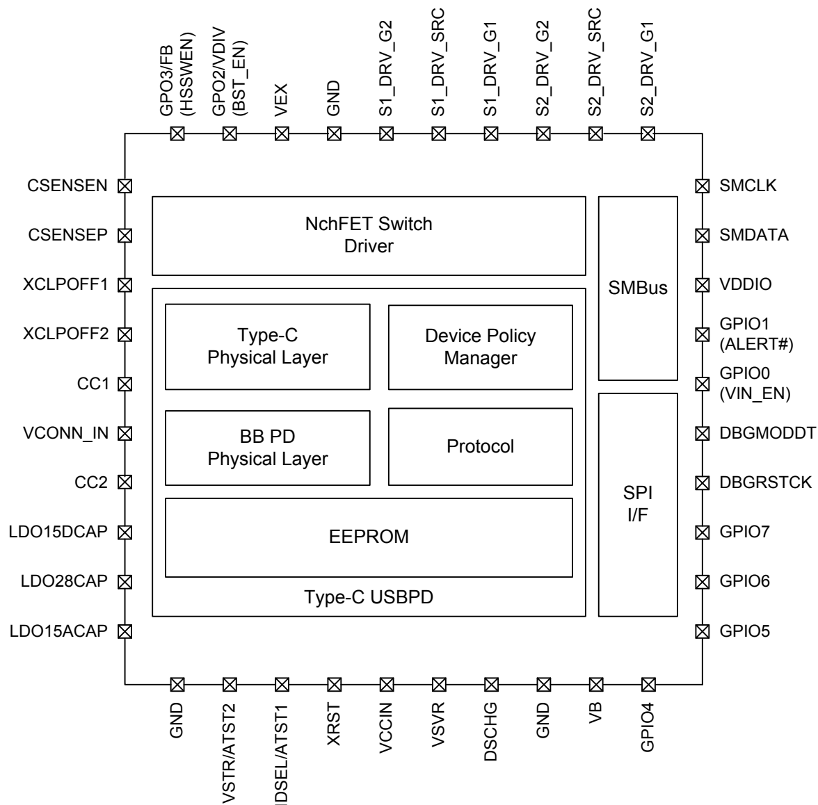
Figure 3-1 Block Diagram
