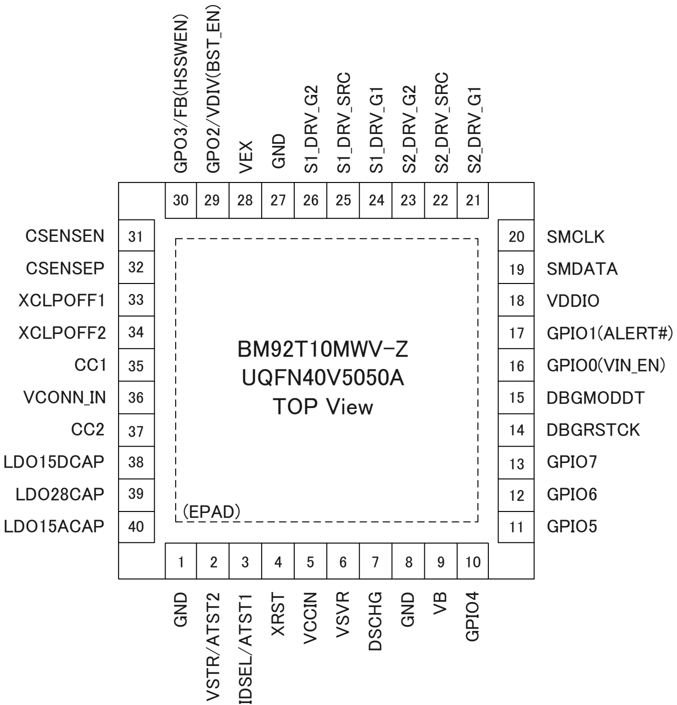
Figure 1-1 Pin configuration
