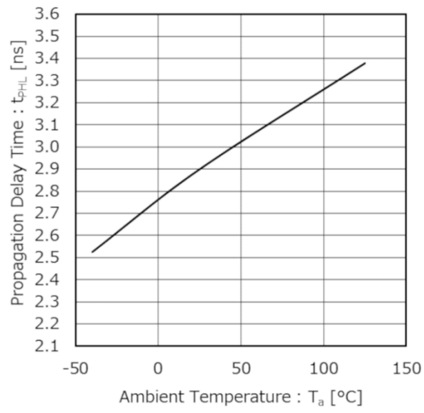
Figure 4. Propagation Delay Time: t_{PHL} vs Ambient Temperature: T_a ( V_{CC} = 3.3\text{ V} )
