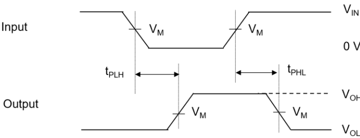
Measurement Circuit and Timing Chart
