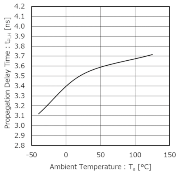
Figure 2. Propagation Delay Time: t_{PLH} vs Ambient Temperature: T_a ( V_{CC} = 3.3\text{ V} )
