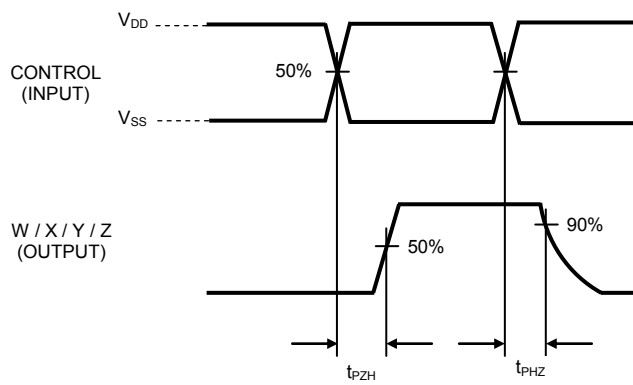
Figure 3. Propagation Delay Time (CONTROL→OUT) ( t_{PLH} , t_{PHL} )
