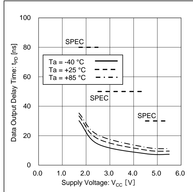
Figure 27. Data Output Delay Time vs Supply Voltage
