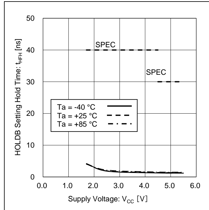
Figure 29. HOLDB Setting Hold Time vs Supply Voltage
