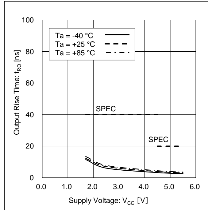
Figure 33. Output Rise Time vs Supply Voltage
