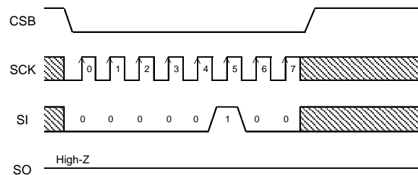
Figure 39. Write Disable Command
