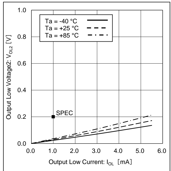
Figure 10. Output Low Voltage2 vs Output Low Current ( V_{CC} = 1.7\text{ V} )
