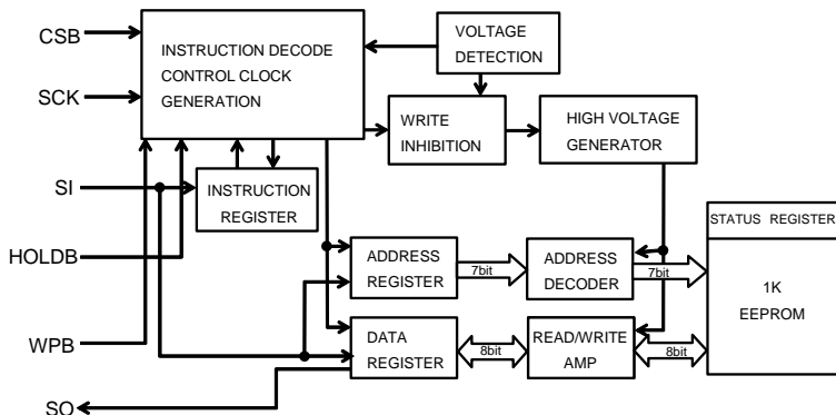
Figure 5. Block diagram
