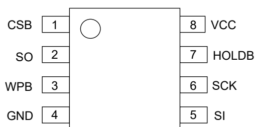
Figure 3-(a). Pin Configuration (SOP8, SOP-J8, TSSOP-B8, MSOP8)
