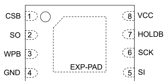
Figure 3-(b). Pin Configuration (VSON08AX2030)
