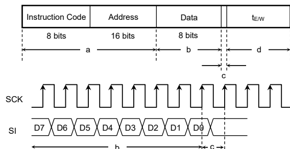
Figure 54. WRITE, WRID, LID Cancel Valid Timing
