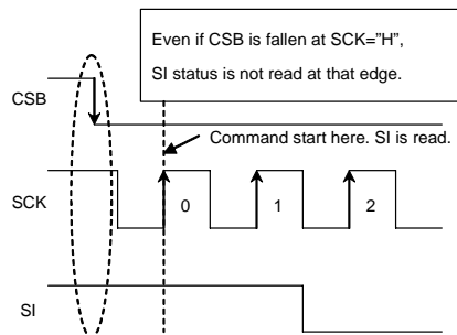
Figure 52. Operating timing
