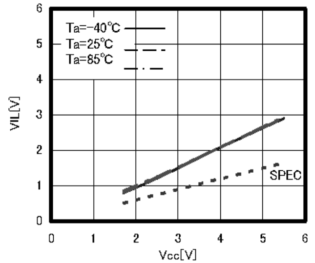
Figure 5. "L" Input Voltage V_{IL} (CSB,SCK,SI,HOLDB, \overline{\text{WP}} )
