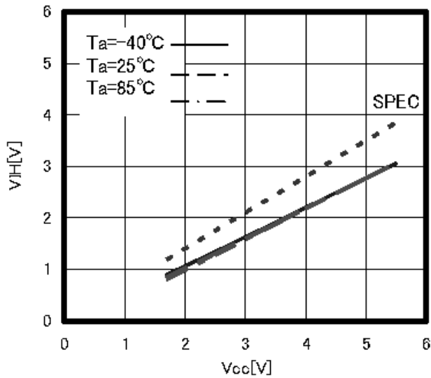
Figure 4. "H" Input Voltage V_{IH} (CSB,SCK,SI,HOLDB, \overline{\text{WP}} )
