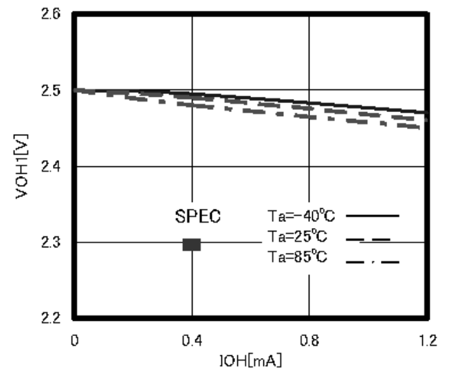
Figure 7. "H" Output Voltage V_{OH1} ( V_{CC}=2.5\text{V} )
