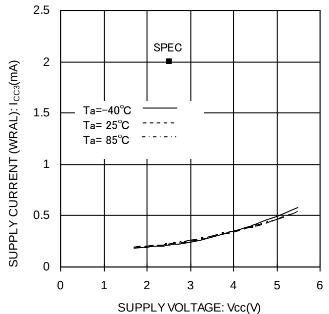
Figure 17. Supply Current (WRAL) vs Supply Voltage ( f_{SK}=1\text{MHz} )
