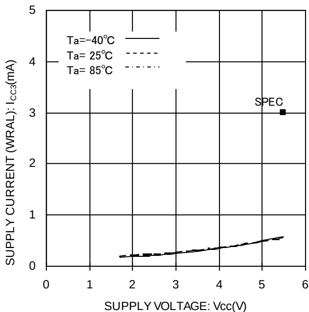
Figure 18. Supply Current (WRAL) vs Supply Voltage ( f_{SK}=3\text{MHz} )
