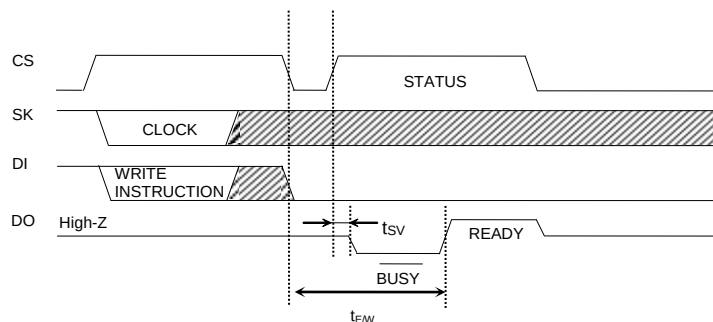
Figure 48. \overline{READY} / \overline{BUSY} STATUS Output Timing Chart
