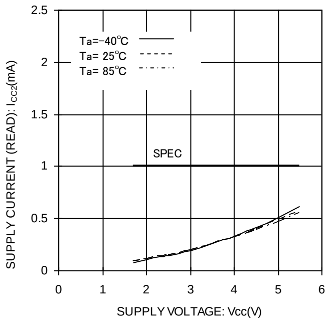
Figure 16. Supply Current (READ) vs Supply Voltage ( f_{SK}=3\text{MHz} )
