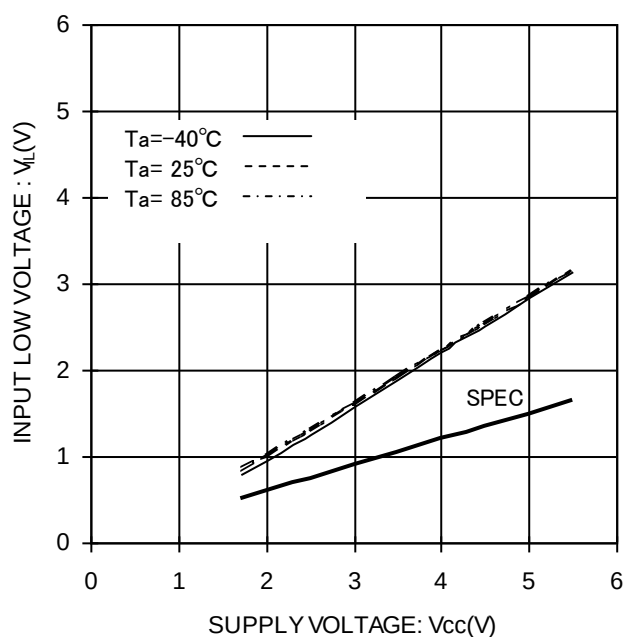
Figure 5. Input Low Voltage vs Supply Voltage (CS,SK,DI,ORG)
