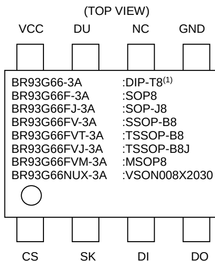
Figure 3. Pin Configuration
