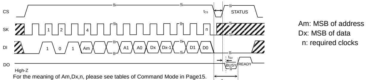
Figure 36. Write Cycle
