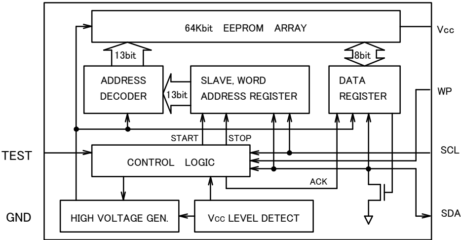
Figure 2. Block Diagram
