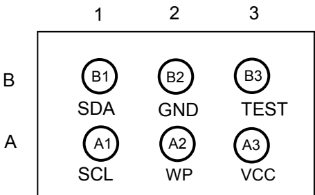
Figure 3. Pin Configuration (BOTTOM VIEW)
