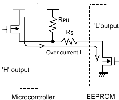
Fig.54-(b) I/O circuit diagram
