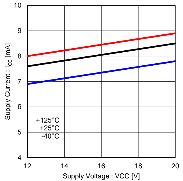
Figure 15. Low Side Drivers Operating Current ( f_{PWM} : 20kHz)
