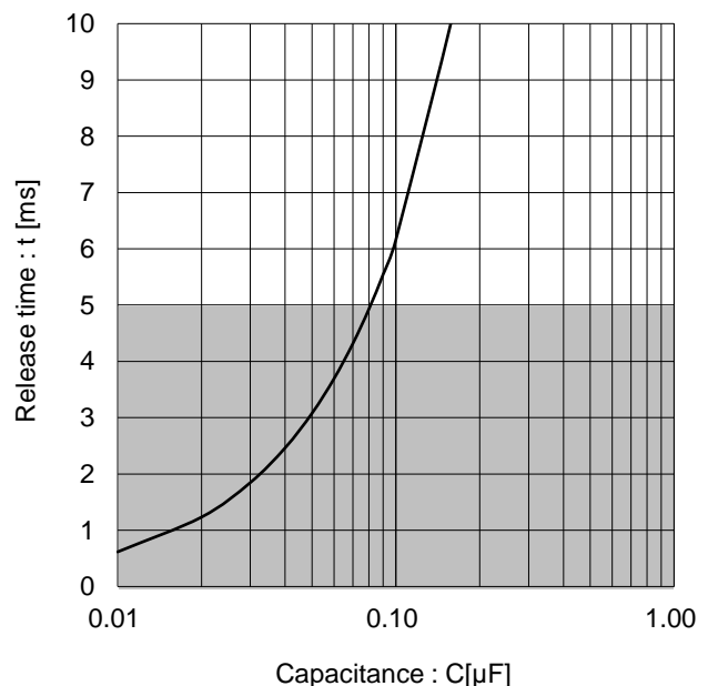
Figure 9. Release Time (Reference Data @R=100k \Omega )
