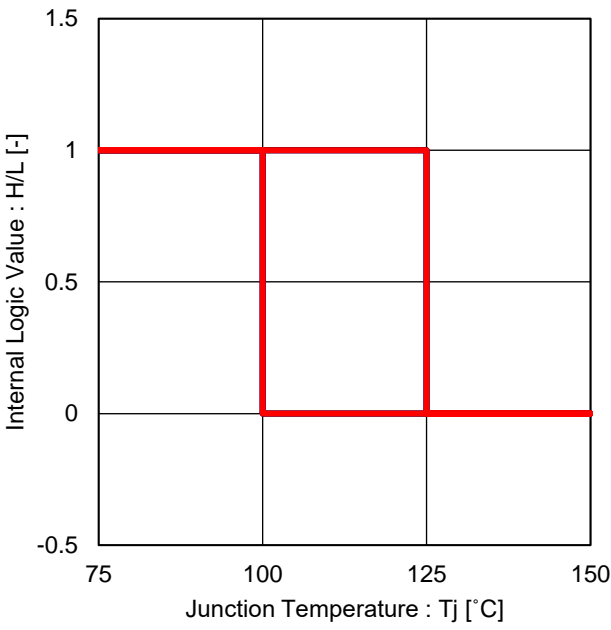
Figure 43 Thermal Shutdown
