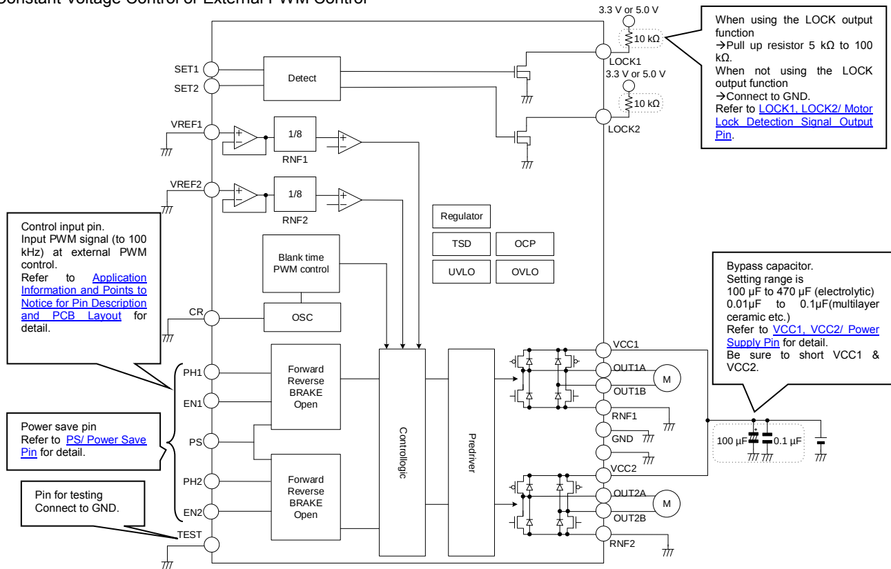
Figure 8. Block Diagram &amp; Application Circuit Diagram
