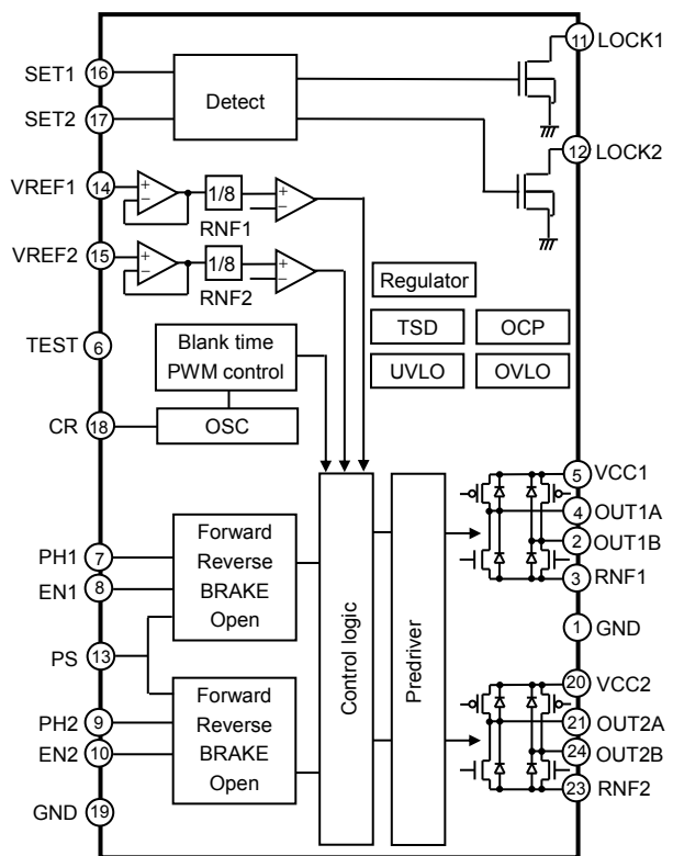
Figure 4. Block Diagram
