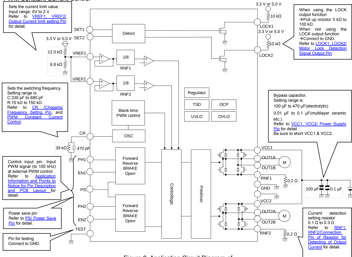
Figure 9. Application Circuit Diagram of Constant Voltage Control or External PWM Control
