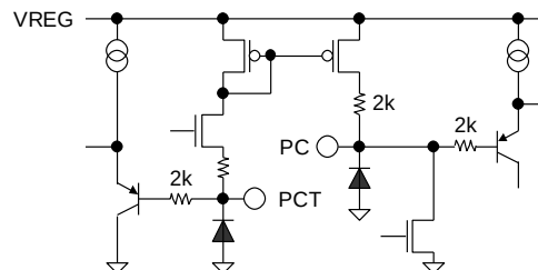
Figure 41. PC, PCT
