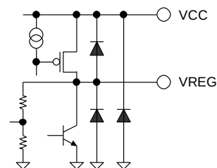
Figure 37. VREG, VCC
