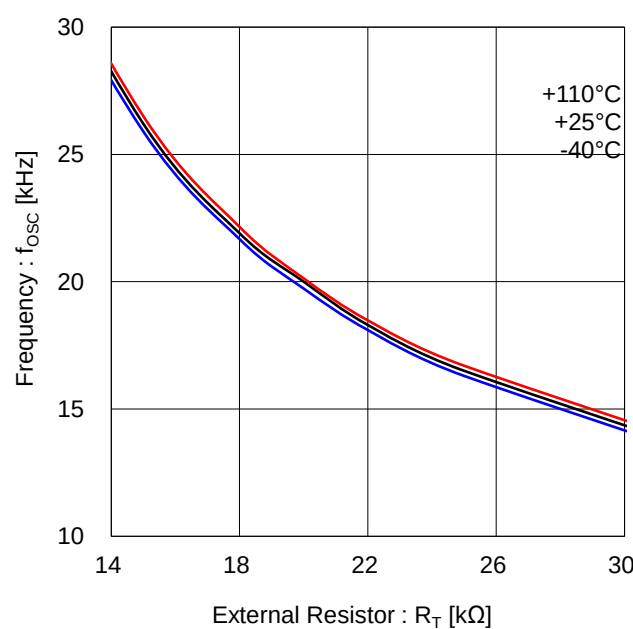
Figure 30. Carrier Frequency vs R_T
