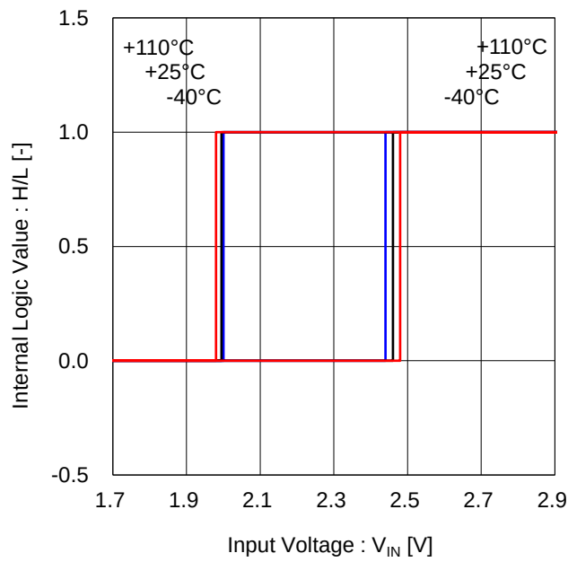
Figure 20. Input Threshold Voltage (CCW, FIB)
