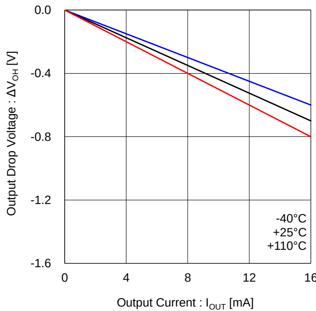
Figure 10. High Side Output Voltage (XH, XL)
