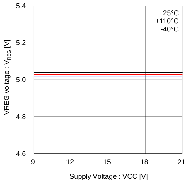
Figure 8. VREG vs VCC
