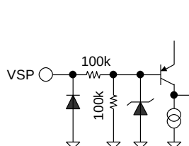
Figure 36. VSP
