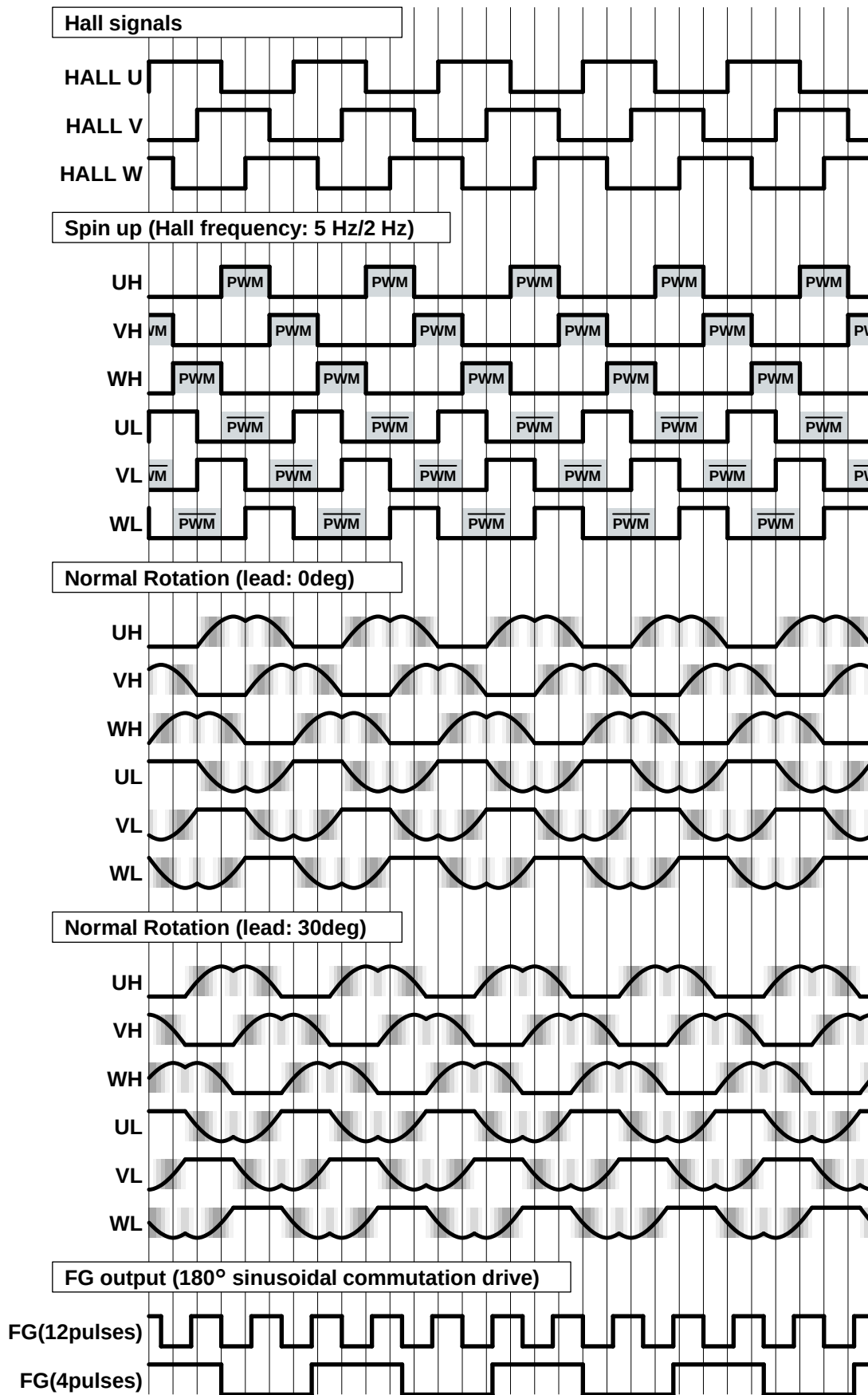
Figure 31. Timing Chart (Clockwise)
