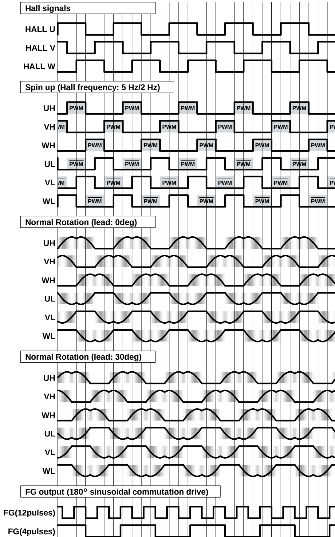
Figure 32. Timing Chart (Counter Clockwise)
