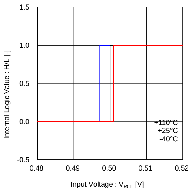
Figure 22. RCL Input Threshold Voltage
