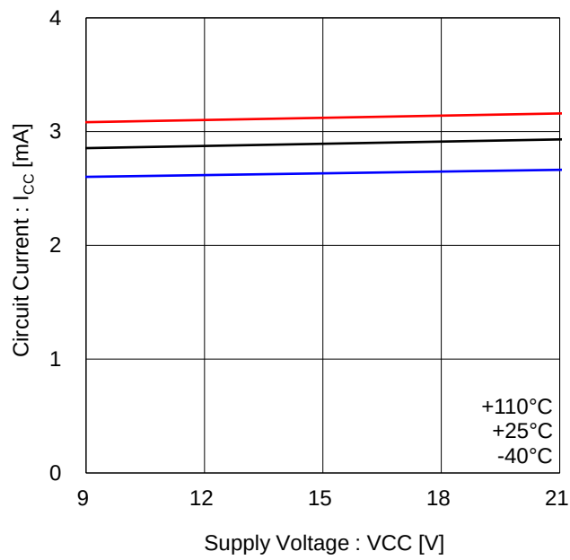
Figure 7. Quiescence Current
