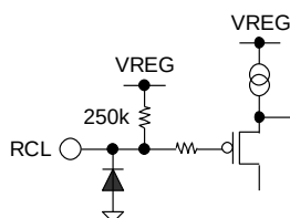
Figure 35. RCL
