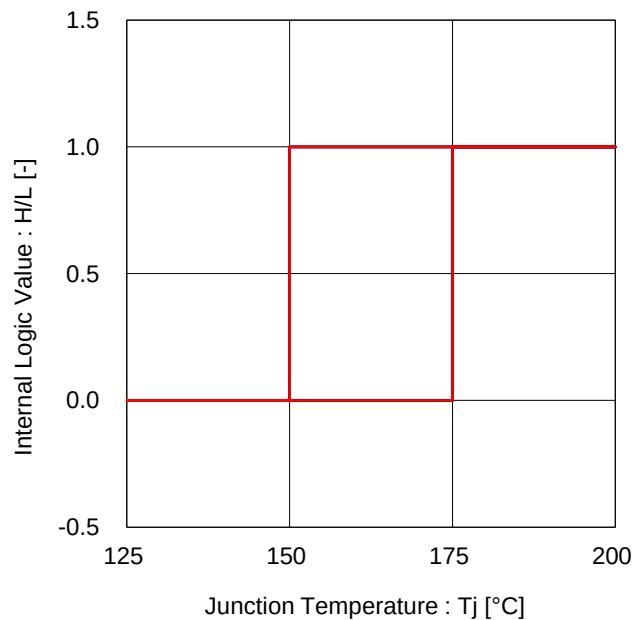
Figure 25. Thermal Shut Down
