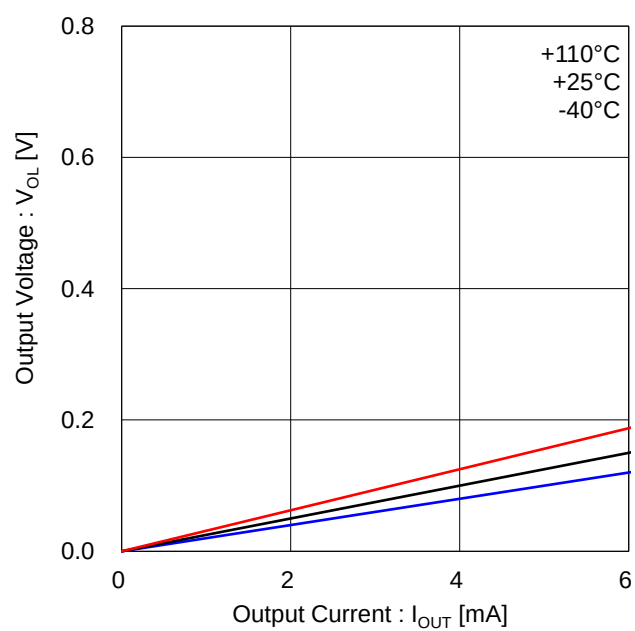
Figure 18. Low Side Output Voltage (FG)
