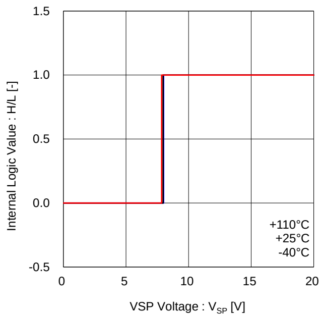
Figure 16. Testing Mode Threshold Voltage
