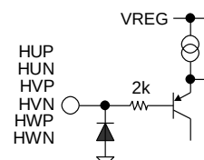
Figure 39. HXP, HXN
