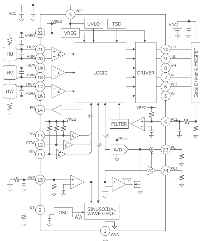
Figure 2. Block Diagram
