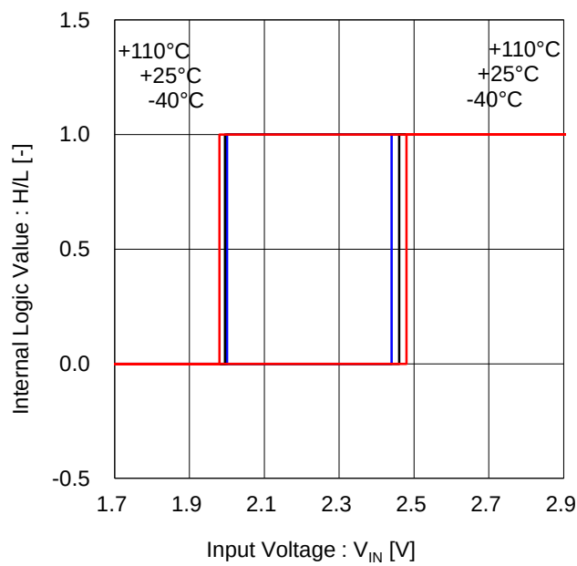
Figure 24. Input Threshold Voltage (FGS)
