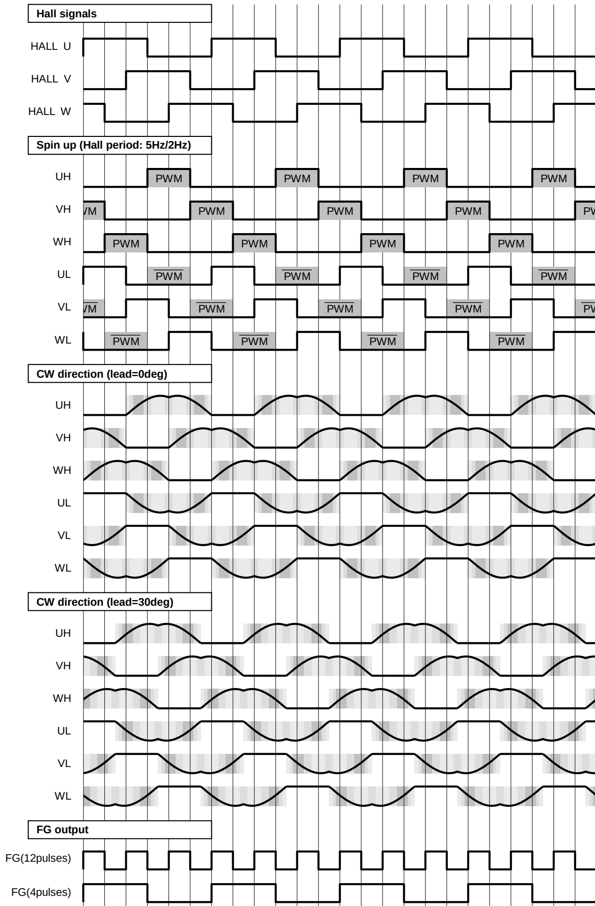
Figure 31. Timing Chart (Clockwise)
