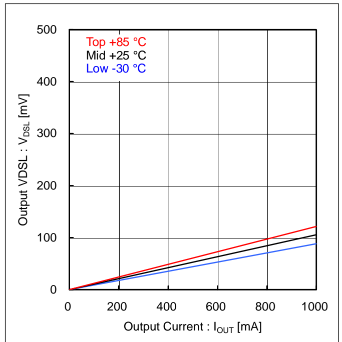
Figure 4. Output VDSL vs Output Current (Output ON-Resistance on low-side, V_M=5 V, V_{CC}=3 V)
