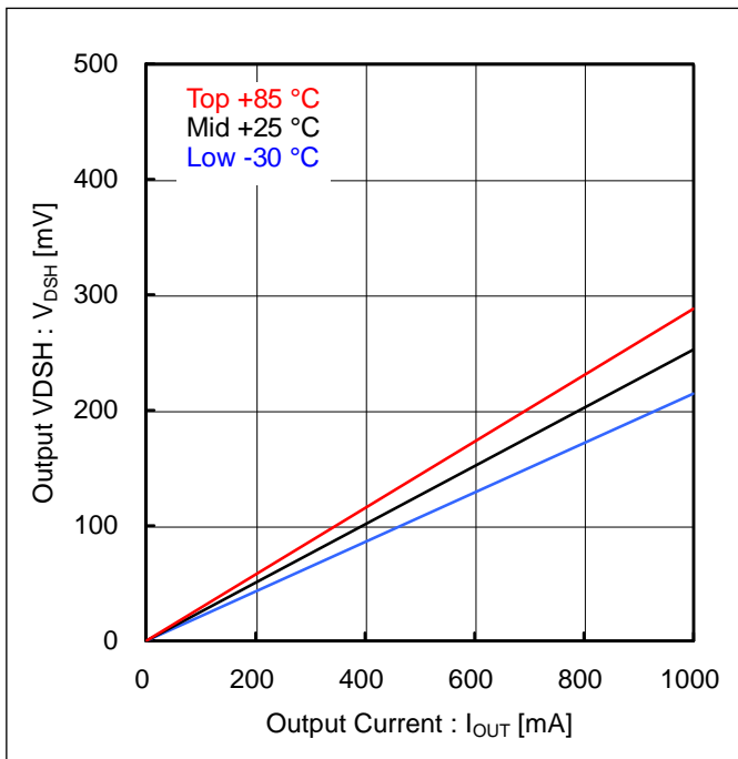
Figure 3. Output VDSH vs Output Current (Output ON-Resistance on high-side, V_M=5 V, V_{CC}=3 V)
