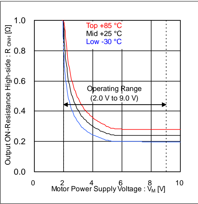
Figure 5. Output ON-Resistance High-side vs Motor Power Supply Voltage (Output ON-Resistance on High-side V_M Dependency, V_{CC}=3\text{ V} )
