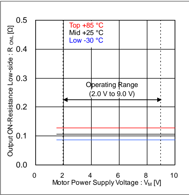
Figure 6. Output ON-Resistance Low-side vs Motor Power Supply Voltage (Output ON-Resistance on Low-side V_M Dependency, V_{CC}=3\text{ V} )
