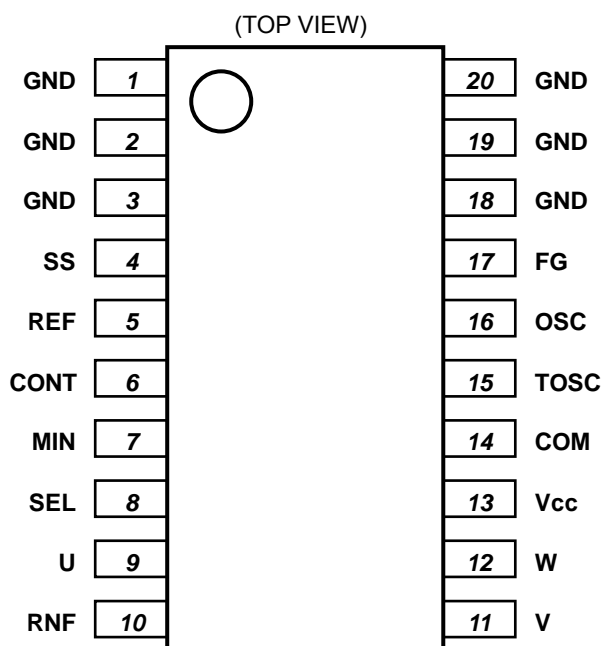
Fig. 1 Pin configuration
