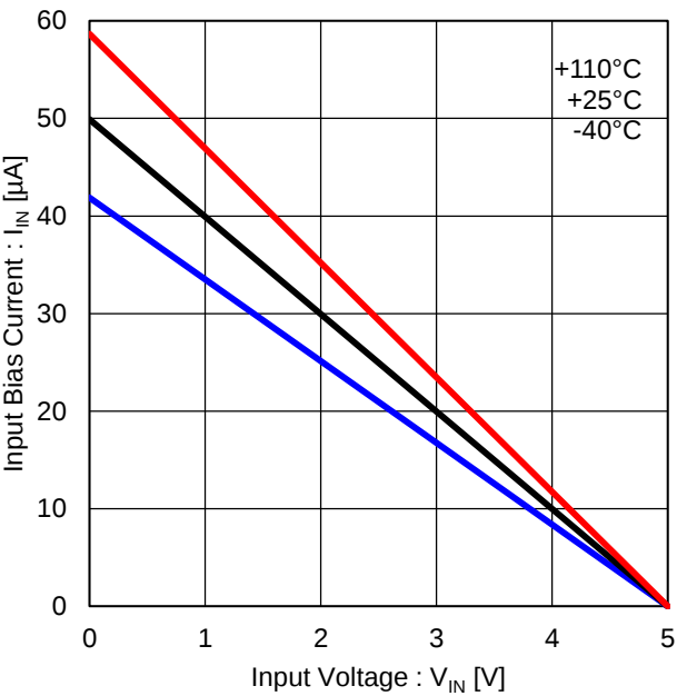
Figure 38. Input Bias Current (CCW, FGS, SQB)
