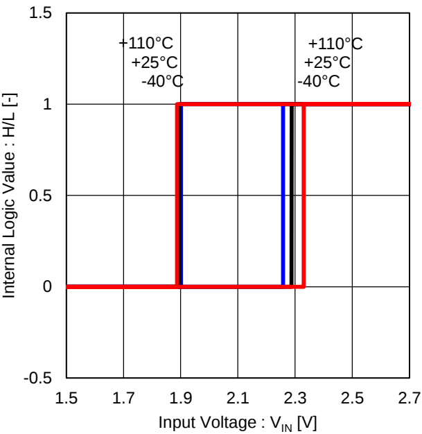
Figure 39. Input Threshold Voltage (CCW, FGS, SQB, FOB)
