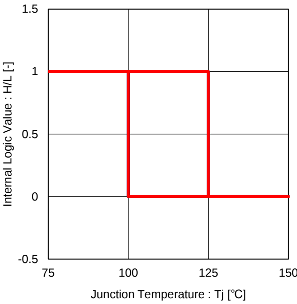
Figure 43 Thermal Shutdown
