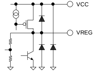
Figure 55. VREG, VCC
