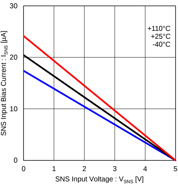
Figure 40. Input Bias Current (SNS)
