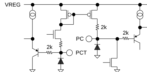
Figure 59. PC, PCT
