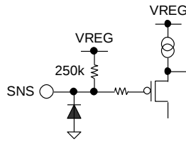
Figure 53. SNS
