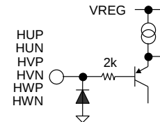
Figure 57. HXP, HXN
