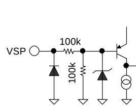
Figure 54. VSP
