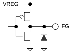
Figure 56. FG
