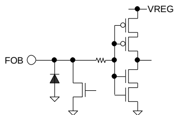
Figure 60. FOB
