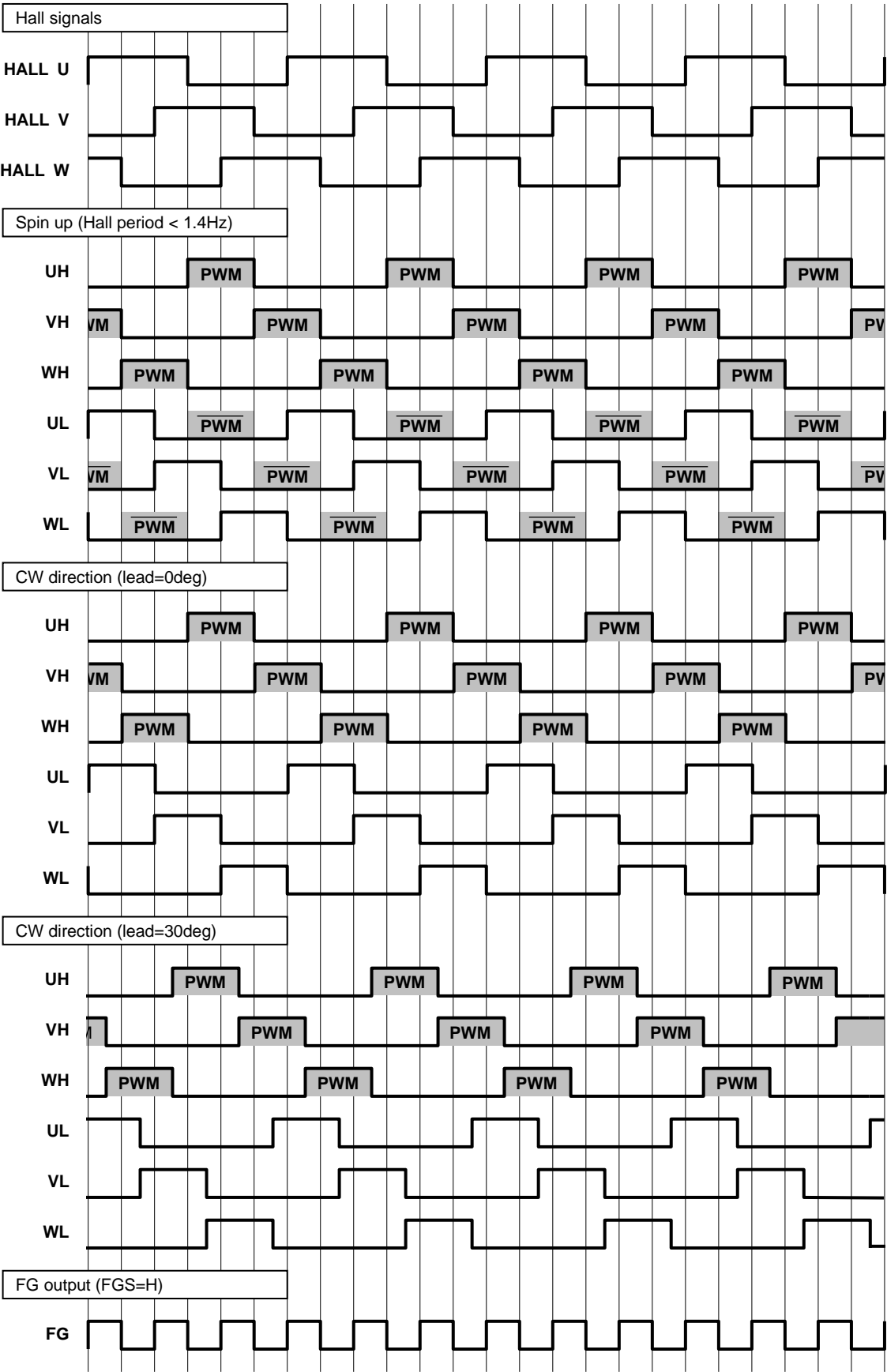
Timing Chart (CW, SQB = L)
