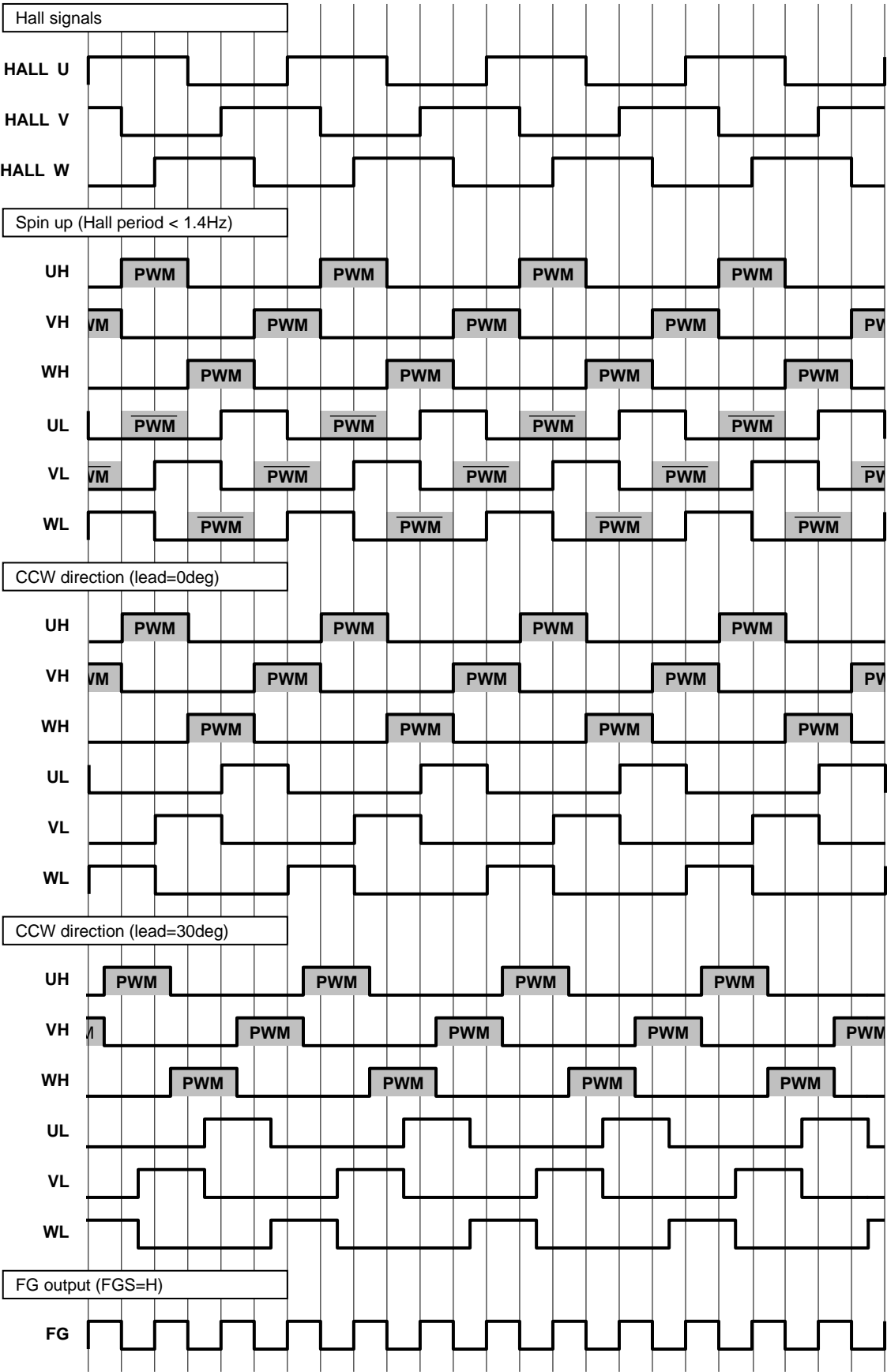
Timing Chart (CCW, SQB = L)
