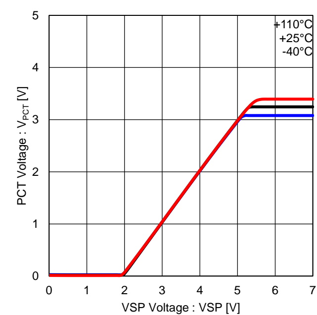
Figure 32. VSP vs PCT Offset Voltage
