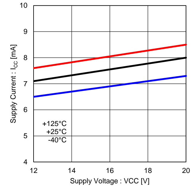
Figure 15. Low Side Drivers Operating Current (f PWM : 20kHz)
