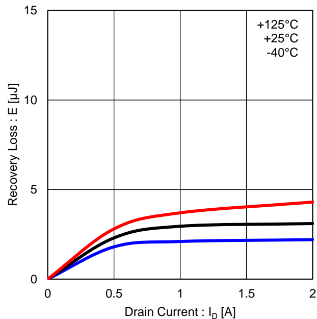
Figure 25. Low Side Recovery Loss (VDC=150V)
