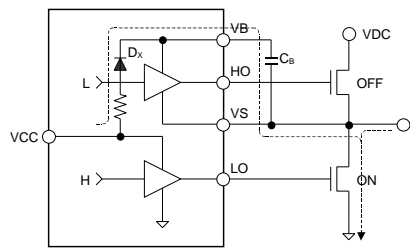
Figure 10. Charging Period
