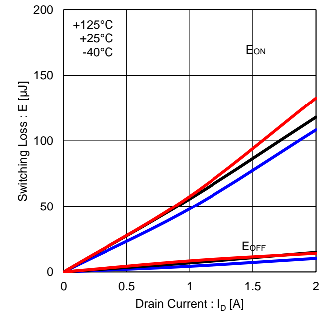
Figure 24. Low Side Switching Loss (VDC=150V)
