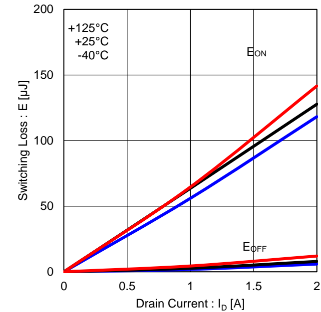
Figure 22. High Side Switching Loss (VDC=150V)
