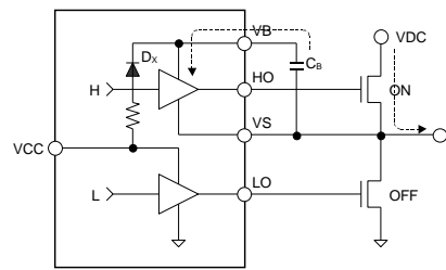
Figure 11. Discharging Period
