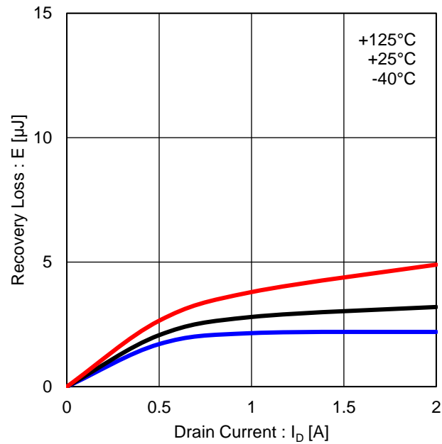
Figure 23. High Side Recovery Loss (VDC=150V)
