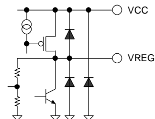
Figure 53. VREG, VCC
