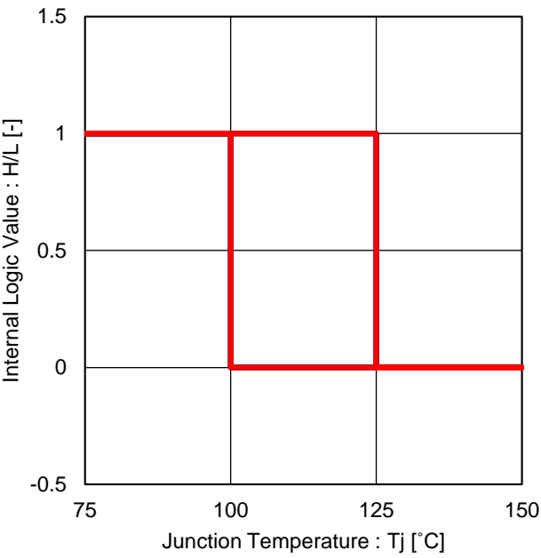
Figure 43 Thermal Shutdown
