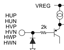
Figure 55. HXP, HXN
