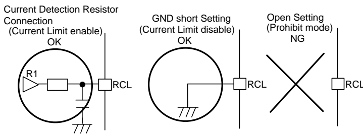
Figure 4. RCL Pin Process
