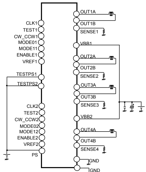
Figure 1. BD63888AEKV Application Circuit Diagram
