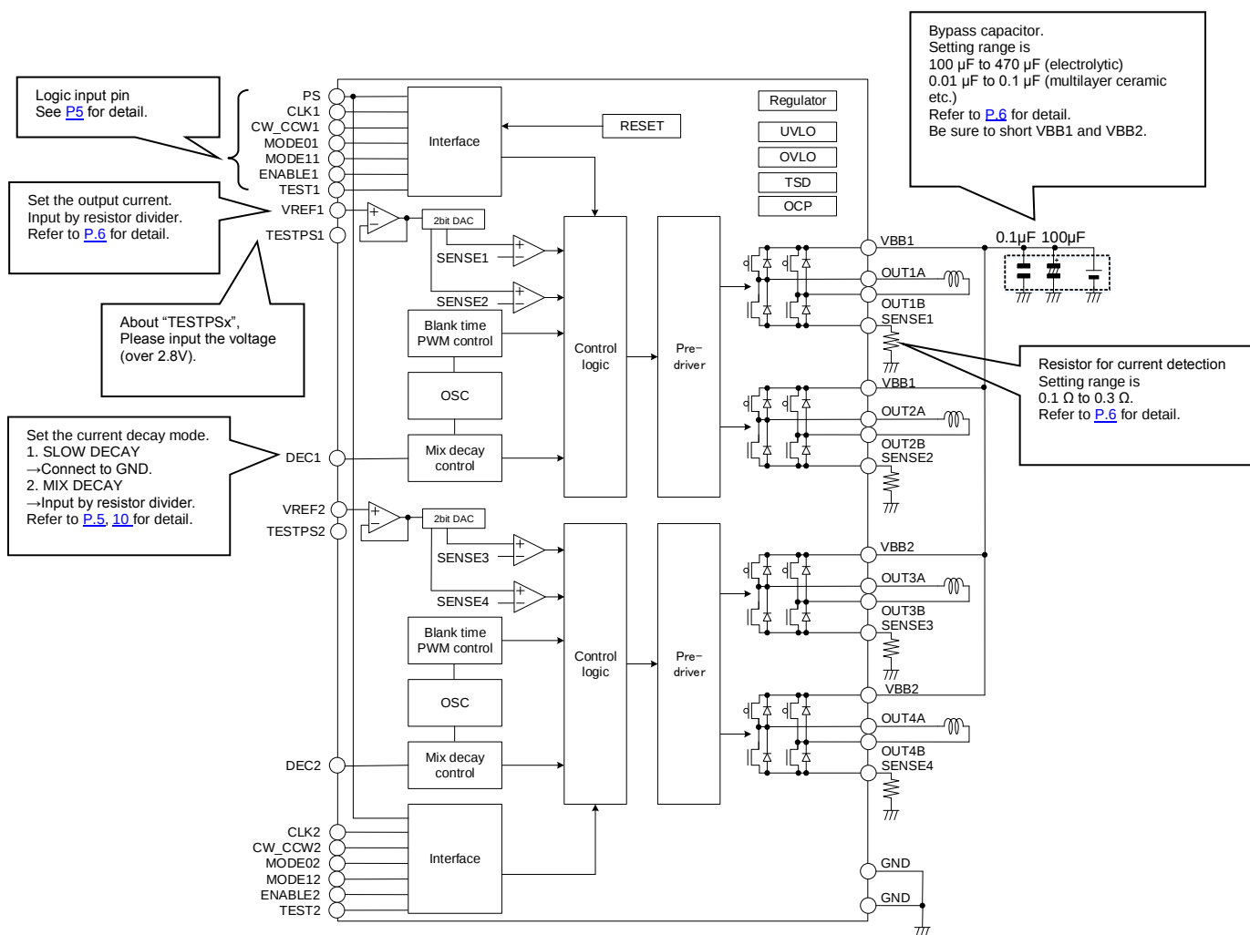
Figure 8. BD63888AEKV Block Diagram and Applied Circuit Diagram
