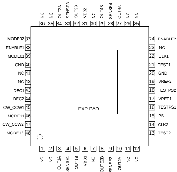
Figure 2. Pins Configuration Diagram
