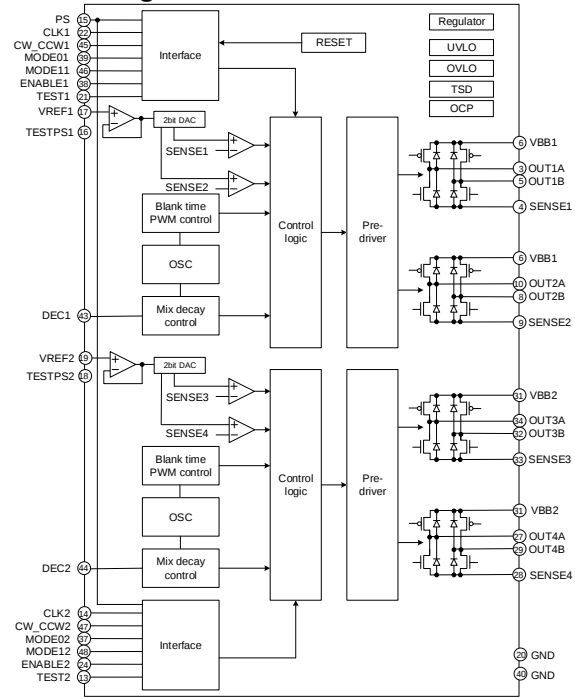
Figure 3. BD63888AEKV Block Diagram
