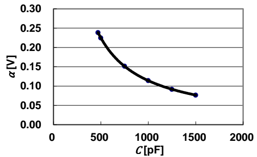
Figure 1. CR Coefficient for Calculation of Discharge Time
