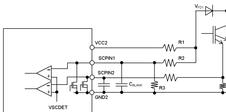
Figure 59. Block Diagram for DESAT
