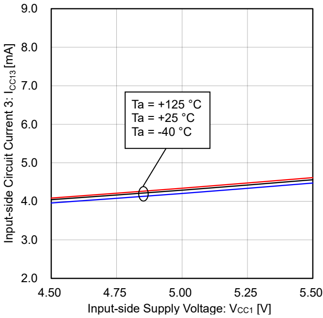
Figure 5. Input-side Circuit Current 3 vs Input-side Supply Voltage
