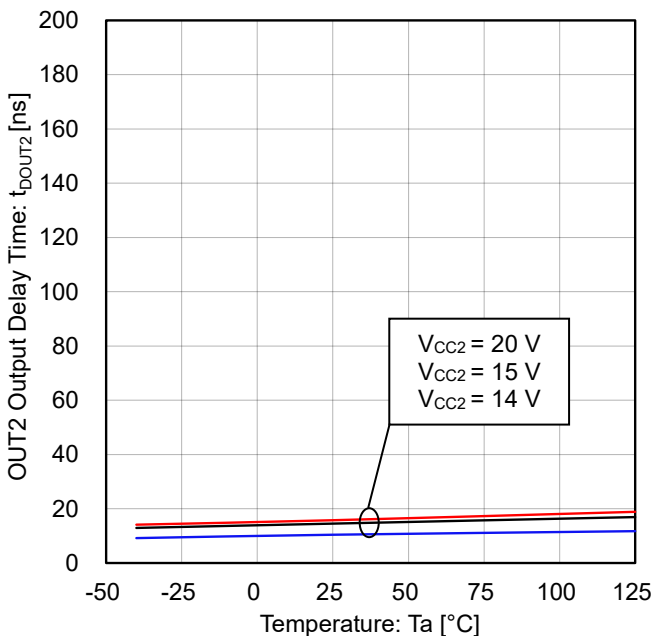
Figure 27. OUT2 Output Delay Time vs Temperature
