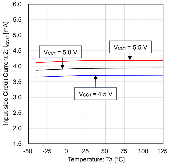
Figure 4. Input-side Circuit Current 2 vs Temperature
