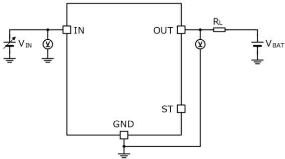
Measurement Circuit for Figure 2
